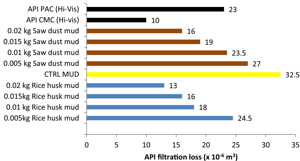
Fig. 4. API filtration loss after 1800 seconds for the formulated water based muds with different concentrations of rice husk and saw dust.
