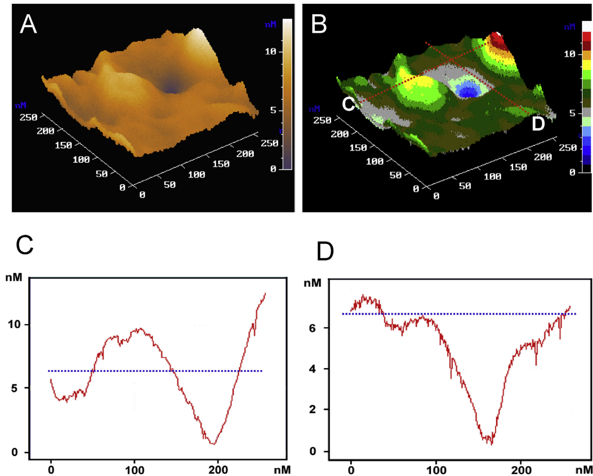
Fig. 4. Exemplary AFM imaging of the third type of membrane pore CH-1-Pore C. (A) Three-dimensional top view of an individual pore in the outer membrane of S. Maccensis from the extracellular side. (B) A contour view of B. (C–D) Profiles of the internal canal indicating the measurable inner diameters. The inverted teepee-shaped structure is apparently segmented into two subunits. The blue dot line indicates the approximately surface height ( R_{\text{mean}} = 6.23 \text{ nM} ) of the outer membrane.
