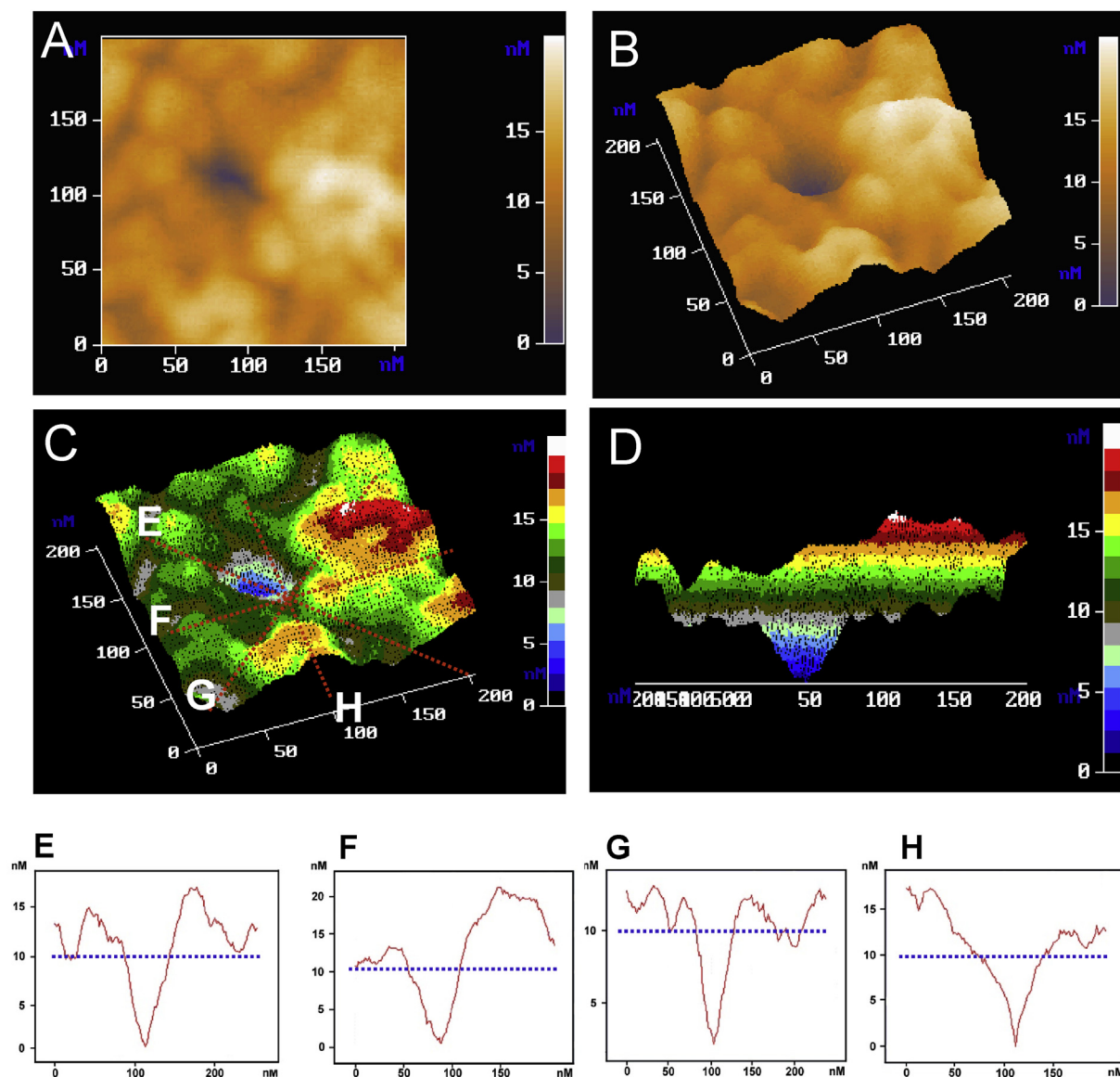
Fig. 2. Exemplary imaging of the first type of membrane pore CH-1-Pore A observed with AFM. (A) and (B) Two- and three-dimensional top view of an individual pore in the outer membrane of S. marcescens from the extracellular side. (C) A contour view of Fig. 2B. (D) View from within the membrane with the extracellular region above and the intracellular region below. (E–H) (depicted from red lines in Fig. 2C). Profiles of the internal canal indicating the measurable inner diameters. The doughnut-like structure displayed in Fig. 2B is segmented into six to eight subunits. The blue dot line indicates the approximately surface height ( R_{\text{mean}} = 9.95 \text{ nm} ) of the outer membrane.
