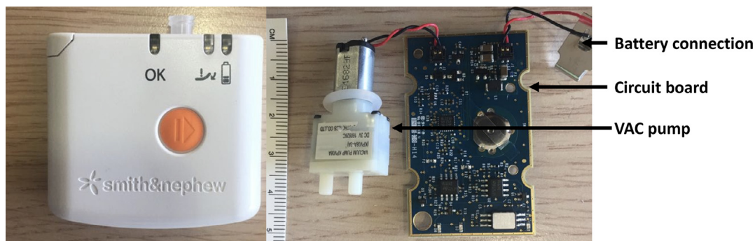
Figure 1 Dismantling of PICO device illustrating circuit board, battery connections and VAC pump.
