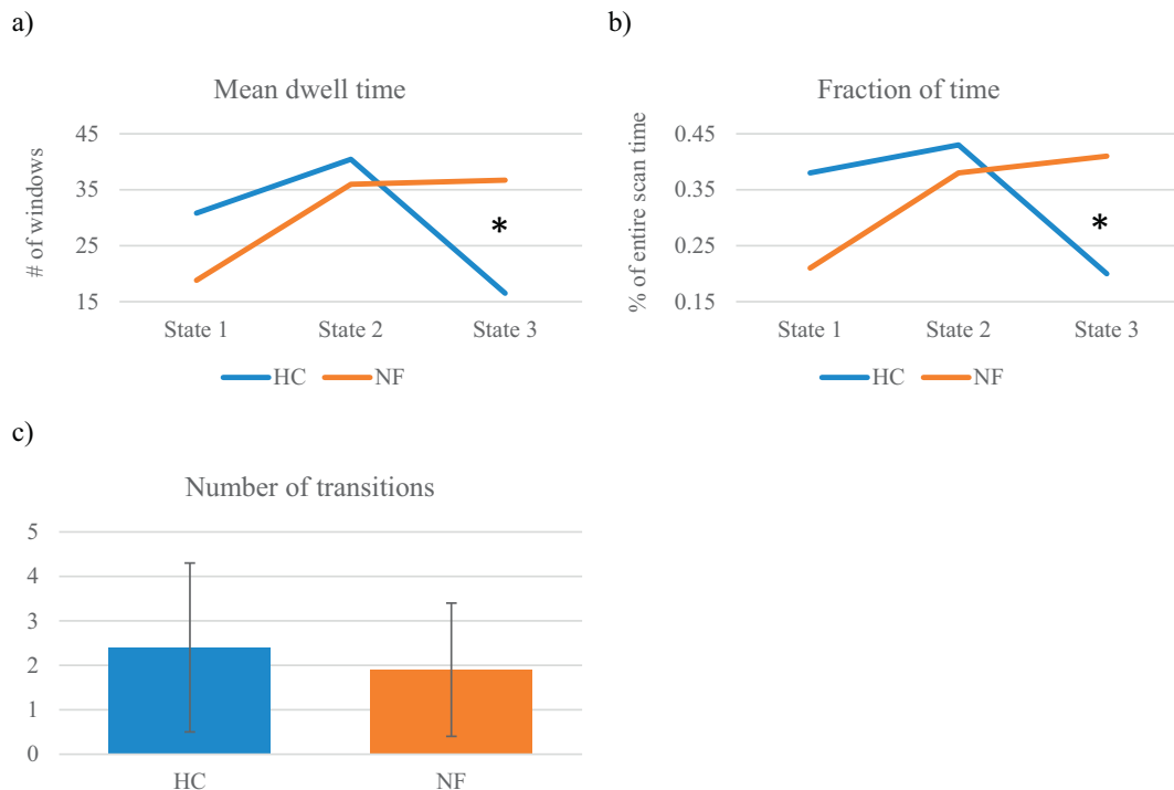
Fig. 3. Plots of a) the mean dwell time, b) fraction of time, and c) the number of transitions for NF1 patients (NF) and Healthy Controls (HC).
