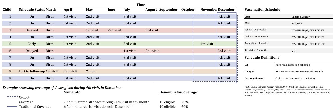
Fig. 3. Example of cohort coverage versus traditional coverage calculations.
