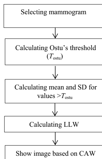
Fig. 3 Flow diagram of filtration and evaluation of mammograms. SD standard deviation, LLW low-level window, CAW computer-aided windowing
