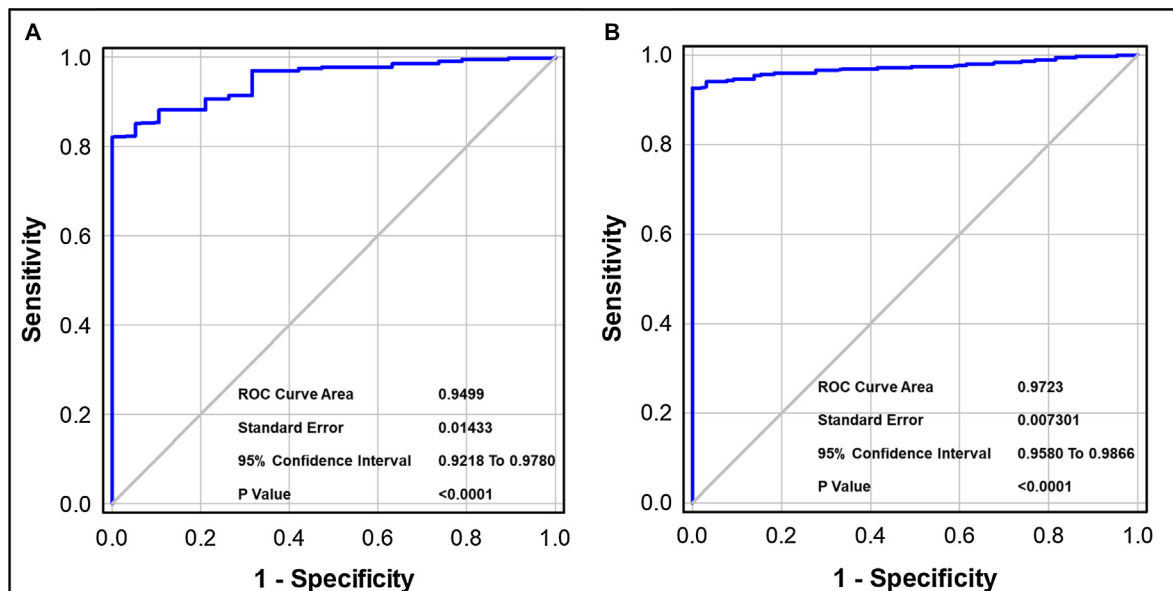
Fig. 4. ROC curve analysis of ELISA and RFFIT. The VNA titres obtained by ELISA was fit with results of RFFIT at two different cut-off values. A. The statistics obtained from the ROC curve analysis at cut-off of 0.5 IU/mL. The curves were plotted by having 1-specificity on 'X axis' and sensitivity on 'Y axis'. The sensitivity denoted the positive coincidence rate and specificity denoted the negative coincidence rate. B. The statistics obtained from the ROC curve analysis at cut-off of 1.5 IU/mL.
