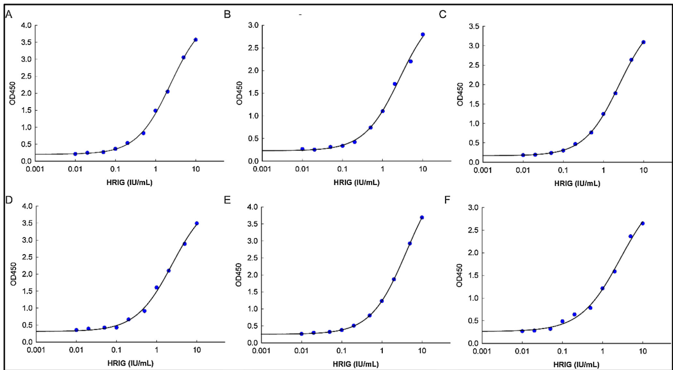
Fig. 2. 4-PL curves of six different test runs using HRIG as the standards. 4-PL curves of the HRIG standards. 100 \mu L of 1:20 diluted HRIG standards (0–10.00 IU/mL spiked in negative human serum) in 20% CS-PBS were added to each well coated with RABV GP. Six curves (A–F) came from six runs altogether performed by three people on two different days. The 4-PL curves were plotted by having concentrations of the HRIG standards on 'X axis' and OD values on 'Y axis' [Equation: y = A2 + (A1 - A2) / (1 + (X/X_0)^P) ].
