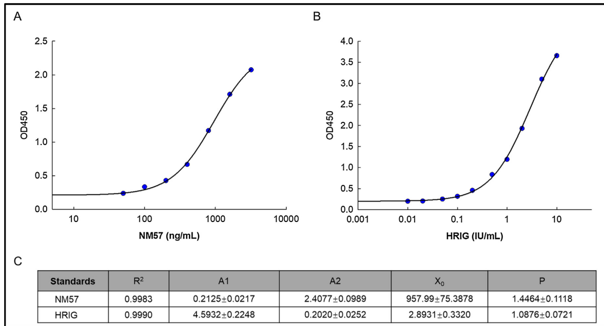
Fig. 1. 4-PL curve using either NM57 or HRIG as standards. 4-PL curves of HuMAb NM57 and HRIG standards. 100 \mu L of 1:20 diluted reference HuMAb NM57 or HRIG standards at different concentrations were added to each well coated with RABV GP. Two 4-PL curves (A & B) was plotted by having concentrations of NM57 or HRIG standards on 'X axis' and OD values on 'Y axis'. [Equation: y = A2 + (A1 - A2) / (1 + (X/X_0)^P) ]. C. The characteristics of two 4-PL curves are listed, A1 indicated the estimation of asymptotes under curves, A2 referred to the estimation of asymptotes on curves, X 0 refers to the concentration for 50% of maximal effect, and P represented the slope of curve.
