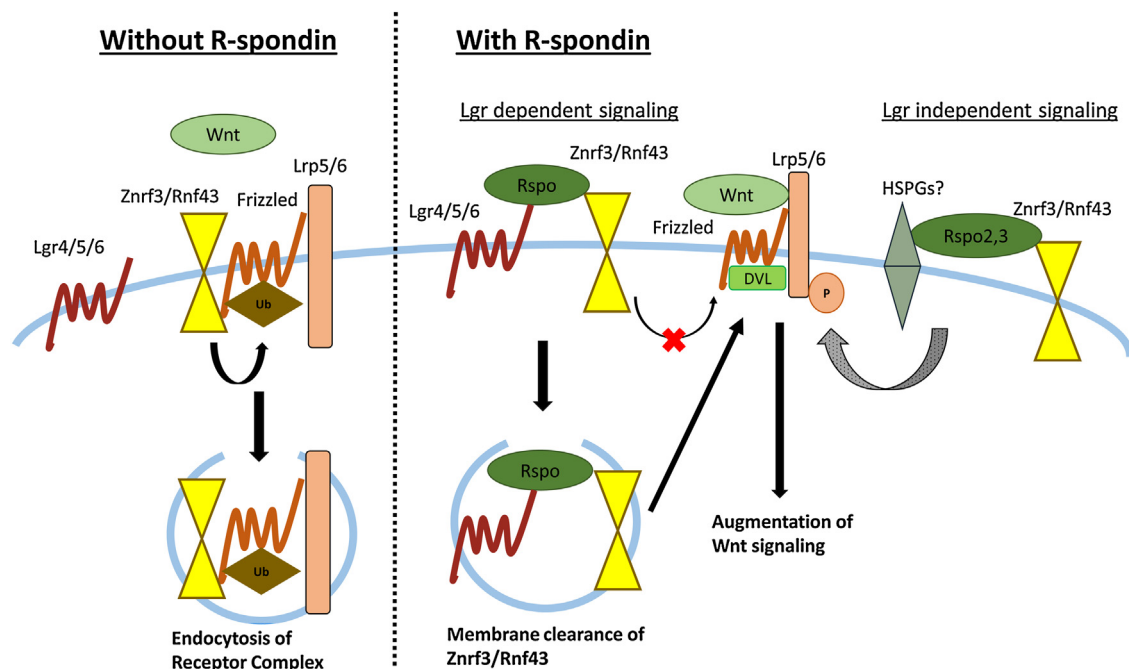
Fig. 2. Schematic diagram of Rspo-induced Wnt signaling augmentation. Without Rspos, Frizzled is ubiquitinated by Znrf3/Rnf43 followed by endocytosis of receptor complex and initiation of Wnt signaling is inhibited. Rspos bind to their receptors Lgr4/5/6 and this complex bind to Znrf3/Rnf43 followed by membrane clearance of these E3 ubiquitin ligases. This allows the receptor complex to initiate downstream signaling, which in turn leads to augmentation of Wnt signaling cascade. Importantly, Rspo2/3 are currently proposed to accelerate Wnt signaling through Lgr-independent signaling.
