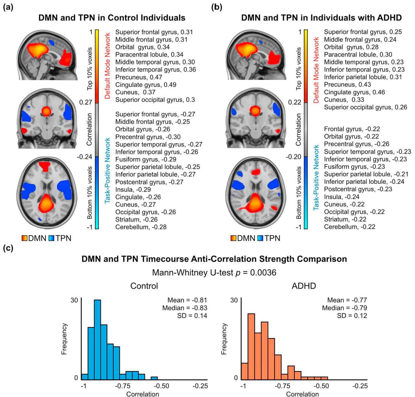
Fig. 1. DMN and TPN in the Control and ADHD groups. Correlation between the mean timecourse of the PCC and every voxel in the brain was calculated. The 10% of voxels most and least correlated with the PCC were defined as the DMN and TPN respectively. (a)Left: The DMN and TPN in the Control group. The DMN comprises all voxels that had correlation with the PCC > 0.27 . The TPN comprises all voxels that had correlation with the PCC < -0.24 . Right: Names of regions in the DMN and TPN in the Control group. (b)Left: The DMN and TPN in the ADHD group. The DMN comprises all voxels that had correlation with the PCC > 0.22 . The TPN comprises all voxels that had correlation with the PCC < -0.20 . Right: Names of regions in the DMN and TPN in the ADHD group. A full list of ROIs in the DMN and TPN, including subdivisions, number of voxels, and strength of correlation with PCC is provided in Supplementary Tables 1 and 2. Compared to the Control group, areas in the DMN had overall lower correlation with the PCC, while areas in the TPN had overall weaker anti-correlation with the PCC. (c) Distributions of anti-correlation strength between DMN and TPN timecourses in all Control ( left ) and ADHD ( right ) scans. Given the non-parametric distributions, a Mann-Whitney U test was performed to compare the strength of anti-correlation, which showed weaker anti-correlation in the ADHD group compared to the control group ( p = .0036 ).
