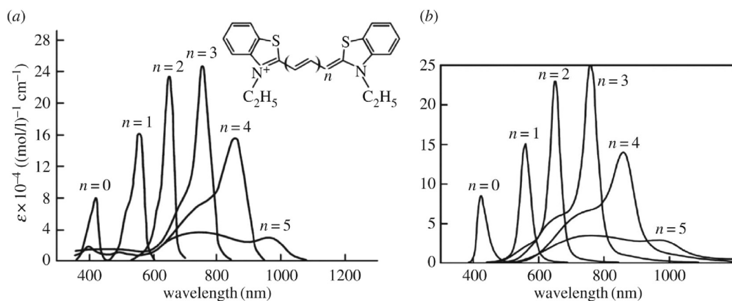
Fig. 1. Experimental [41, 43] (a) and theoretical [12] (b) monomer's optical absorption spectra dependent on the length of the polymethine chain (thiapolymer-thinecyanine in methanol at room temperature; \epsilon is the extinction coefficient) [15, 18, 19]. (Original citation) — Reproduced by permission of The Royal Society of Chemistry.
