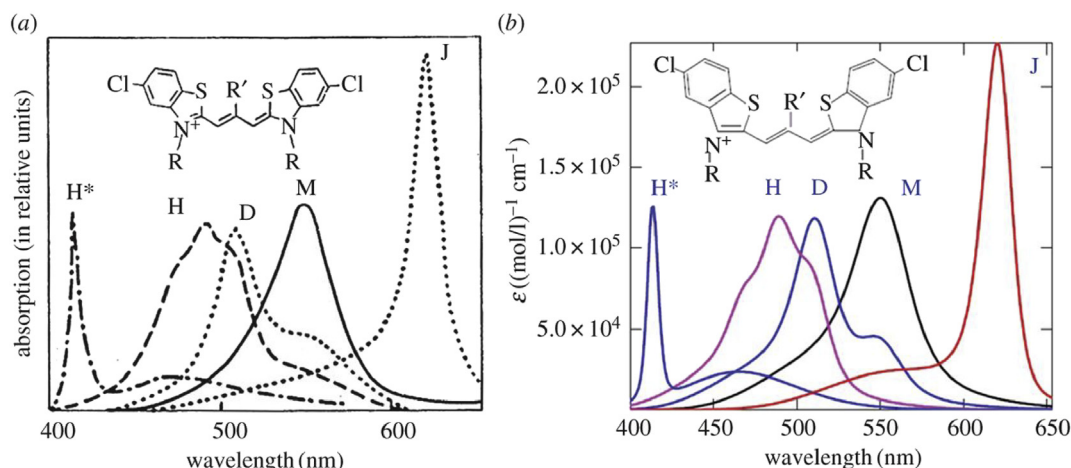
Fig. 2. Theoretical optical absorption spectra [18, 19, 29, 35] (b) in thiapolymer-thinecyanines adjusted to the fundamental experimental data (a) on polymethine dye monomers (M), dimers (D), H-, H*, and J-aggregates [43].
