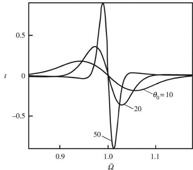
Fig. 3. The dynamics of quantum-classical transitions in the neighborhood of the singular point ( \bar{\Omega} = 1 , \theta_0 = \infty ) [ \Delta = E , \gamma = 0 ] is demonstrated by the behaviour of the quantity t = t(\bar{\Omega}, \theta_0) (see Eq. (144)) [11]. For simplification, it is formally assumed here that J_2 - J_1 = 0 . Then \Theta^{-1} = \hbar\Omega/E \equiv \bar{\Omega} . The following system parameters are used: J_1 = 5 eV, E = 1 eV, \mu = m_e , \omega = 5 \times 10^{13} \text{ s}^{-1} and L = L^* \approx 0.44 nm (transferon resonance, Eq. (161)).
