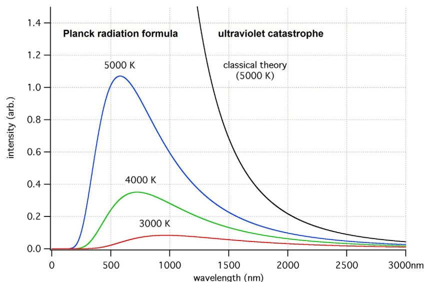
Fig. 5. Distribution function of black light \phi(\lambda, T) (Eq. (165)).
