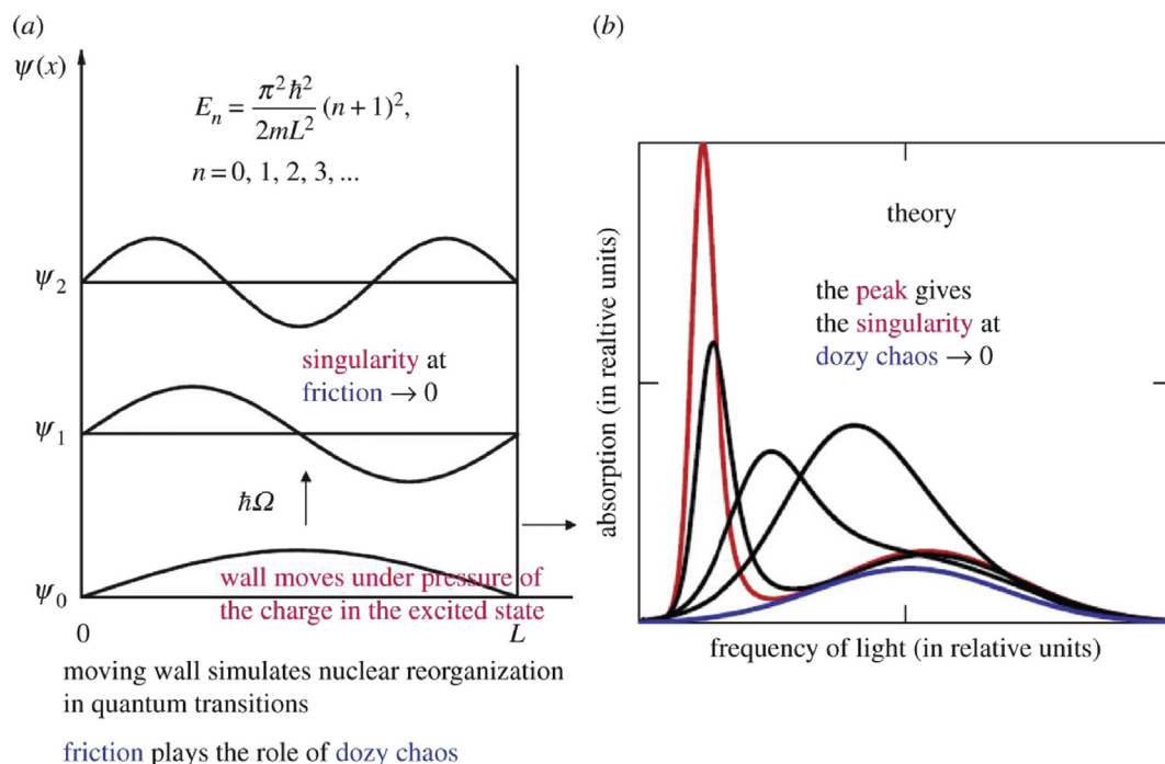
Fig. 4. Singularity in the rate of molecular “quantum” transitions: a potential box with a moveable wall (a) and the optical absorption band shape dependant on the dozy chaos accessible to a certain “quantum” transition (b); the pronounced peak (J-band) matches the least dozy chaos [15, 18]. (Original citation) — Reproduced by permission of The Royal Society of Chemistry.
