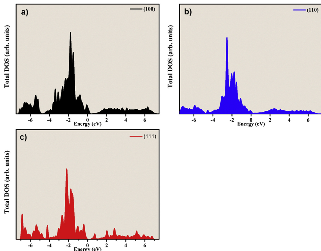
Fig. 5. Total density of states of the a) 100, b)110 and c)111 \text{Cu}_2\text{O} surface models.
