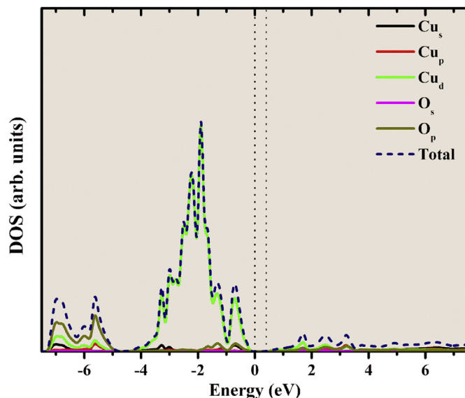
Fig. 2. Projected density os state of \text{Cu}_2\text{O} bulk.
