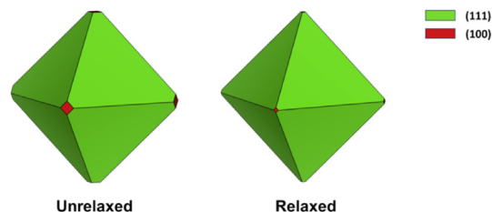
Fig. 6. Wulff crystals of the unrelaxed and relaxed structure of \text{Cu}_2\text{O} .
