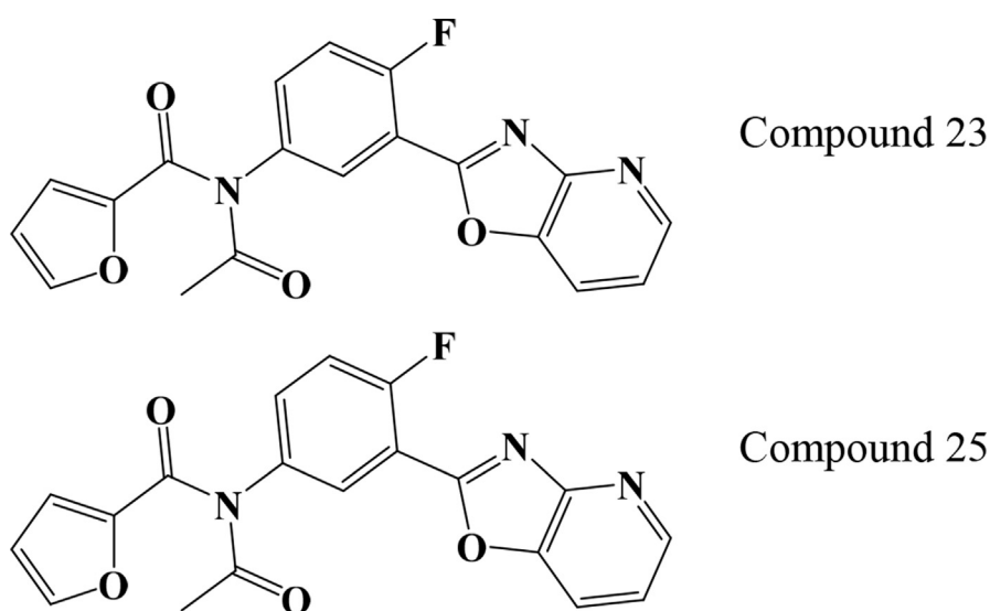
Fig. 6. Chemical structures of the outsiders compounds.
