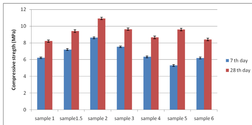
Fig. 5. Compressive Strength of the Pozzolana-ALS cements.
