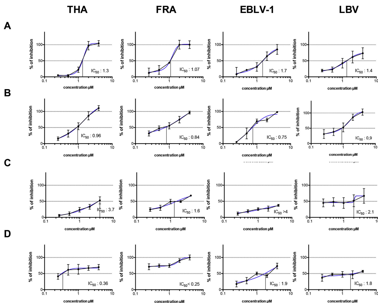
Fig. 3. Spectrum of activity of pyrimethamine and ribavirin. The spectrum of activity of pyrimethamine and ribavirin alone or in combination was tested using 4 field isolates, Tha, FRA, EBLV-1 & LVB, which belongs to 3 different species of lyssavirus. Cells were infected with 200 UFF of virus. Graphs showed the mean \pm SEM of three independent experiments. A: Pyrimethamine at different concentrations. B: Pyrimethamine at different concentrations combined with 2 \mu M of ribavirin. C: Ribavirin at different concentrations. D: Ribavirin at different concentrations combined with 1 \mu M of pyrimethamine.
