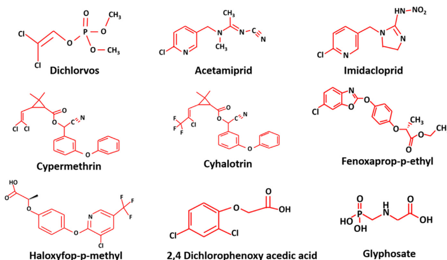
Fig. 1. Structure of tested some pesticides.
