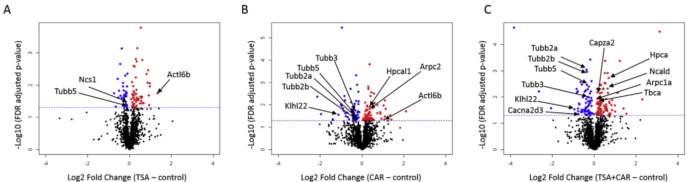
Fig. 3. Volcano plots depicting protein expression in each of the treatments; TSA (A), CAR (B), and TSA + CAR (C). The \log_2 fold change (x-axis) and -\log_{10} p-value (y-axis) of each protein identified in each of the comparisons is shown. Significant proteins that are either up- or down-regulated in the treatment are highlighted in red and blue, respectively. The horizontal line indicates a p-value of 0.05.
