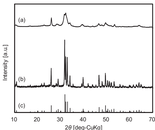
Fig. 2. XRD patterns of the synthesized HA hollow microspheres (a), commercially available HA microrods (b), and HA standard data (ICDD 9–432) (c).
