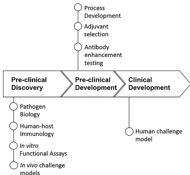
Fig. 3. Zika case study summary. As a relatively neglected pathogen until recently, much of the bottlenecks identified are in the pre-clinical discovery phase, which requires antigen identification and development of assays and challenge models. The need for a new vaccine also incurs bottlenecks in the pre-clinical development phase and in clinical development.
