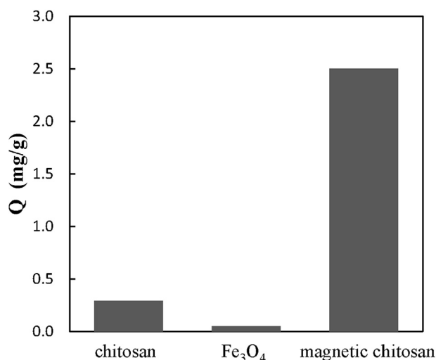
Fig. 5. Adsorption capacity of chitosan, \text{Fe}_3\text{O}_4 and magnetic chitosan for Hg(II) adsorption.
