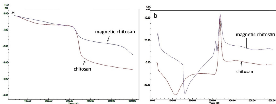
Fig. 4. TGA (a) and DSC (b) curves of chitosan and magnetic chitosan.
