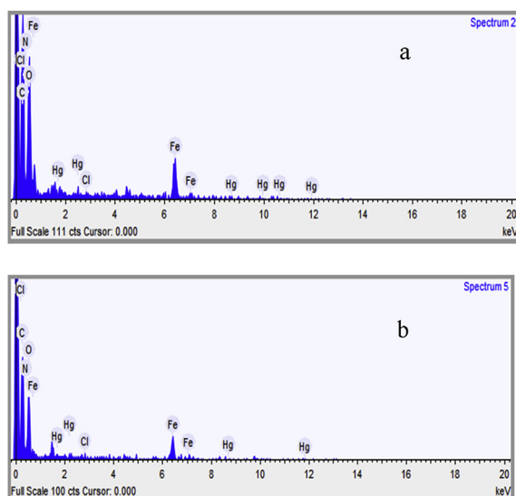
Fig. 9. EDS analysis of magnetic chitosan before (a) and after (b) adsorption.
