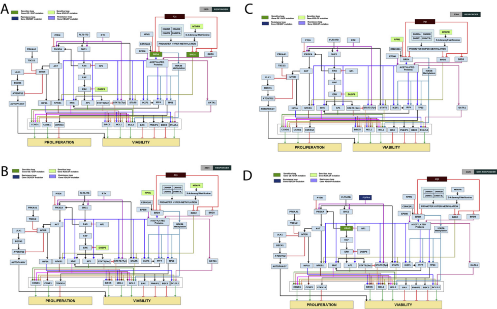
Fig. 4. A-D: Computer-simulated patient-specific network maps and digital response to JQ1. Patient specific network maps were generated using CBM modeling. Patient 2305 (A) and 2304 (B) are representative examples of profiles predicted to be sensitive to JQ1 as measured by the in-silico AML disease inhibition score. Patient 4006 (C) and 1126 (D) are representative examples of profiles predicted to be resistant to JQ1 as measured by the in-silico AML disease inhibition score. Boxes highlighted in light green represent gene mutations leading to protein loss of function or knock-down contributing to drug sensitivity. Boxes highlighted in darker green represent gene mutations leading to protein gain of function or over-expression contributing to drug sensitivity. Boxes highlighted in purple represent gene mutations leading to loss of function or knock-down of proteins contributing to drug resistance, and boxes highlighted in dark blue represent gene mutations leading to protein gain of function or over-expression contributing to drug resistance. (For interpretation of the references to colour in this figure legend, the reader is referred to the web version of this article).
