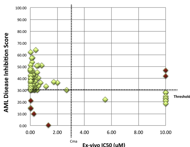
Fig. 2. Illustration of AML disease inhibition score associations with ex vivo JQ1 IC_{50} values. A scatterplot representing ex vivo determined IC_{50} (X-axis) and virtually simulated disease inhibition scores of JQ1 (Y-axis). Cut-offs to determine sensitivity and resistance were determined empirically. For CBM response predictions (Y-axis), 30% disease inhibition was chosen as the threshold for response (horizontal threshold dotted line). A disease inhibition score > 30\% is classified as a responder, or sensitive to JQ1, while a disease inhibition score < 30\% is classified as a non-responder, or resistant to JQ1. For ex vivo IC_{50} values (X-axis), the C_{max} of JQ1 was calculated from a previous study and used as the threshold for response. [11] (Vertical C_{max} dotted line) IC_{50} < 2.7\mu M was considered sensitive, and IC_{50} > 2.7\mu M was considered resistant. The green diamonds indicate the responder and non-responder predictions that matched with the ex vivo response, while the red diamonds indicate false negatives and false positive predictions. Green diamonds (light) vs. red diamonds (Dark) (For interpretation of the references to colour in this figure legend, the reader is referred to the web version of this article).
