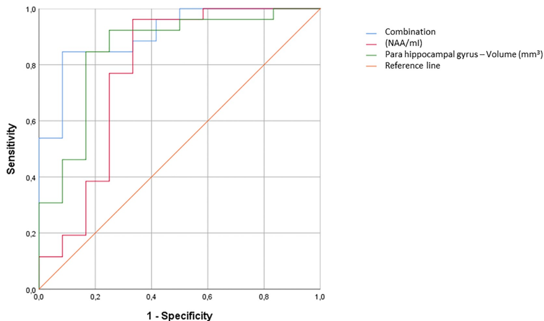
Fig. 3. ROC curves for baseline NAA/ml, baseline brain volumetry (parahippocampal gyrus) and their combination as predictors of conversion from MCI to AD. NAA/ml: AUC = 0.779; sensitivity 76.9%; specificity 75.0%; PPV 87.0%. Parahippocampal gyrus volume: AUC = 0.853; sensitivity 84.6%; specificity 83.3%; PPV 91.7%. Combination of parameters: AUC = 0.910; sensitivity 84.6%; specificity 91.7%; PPV 95.6%.
