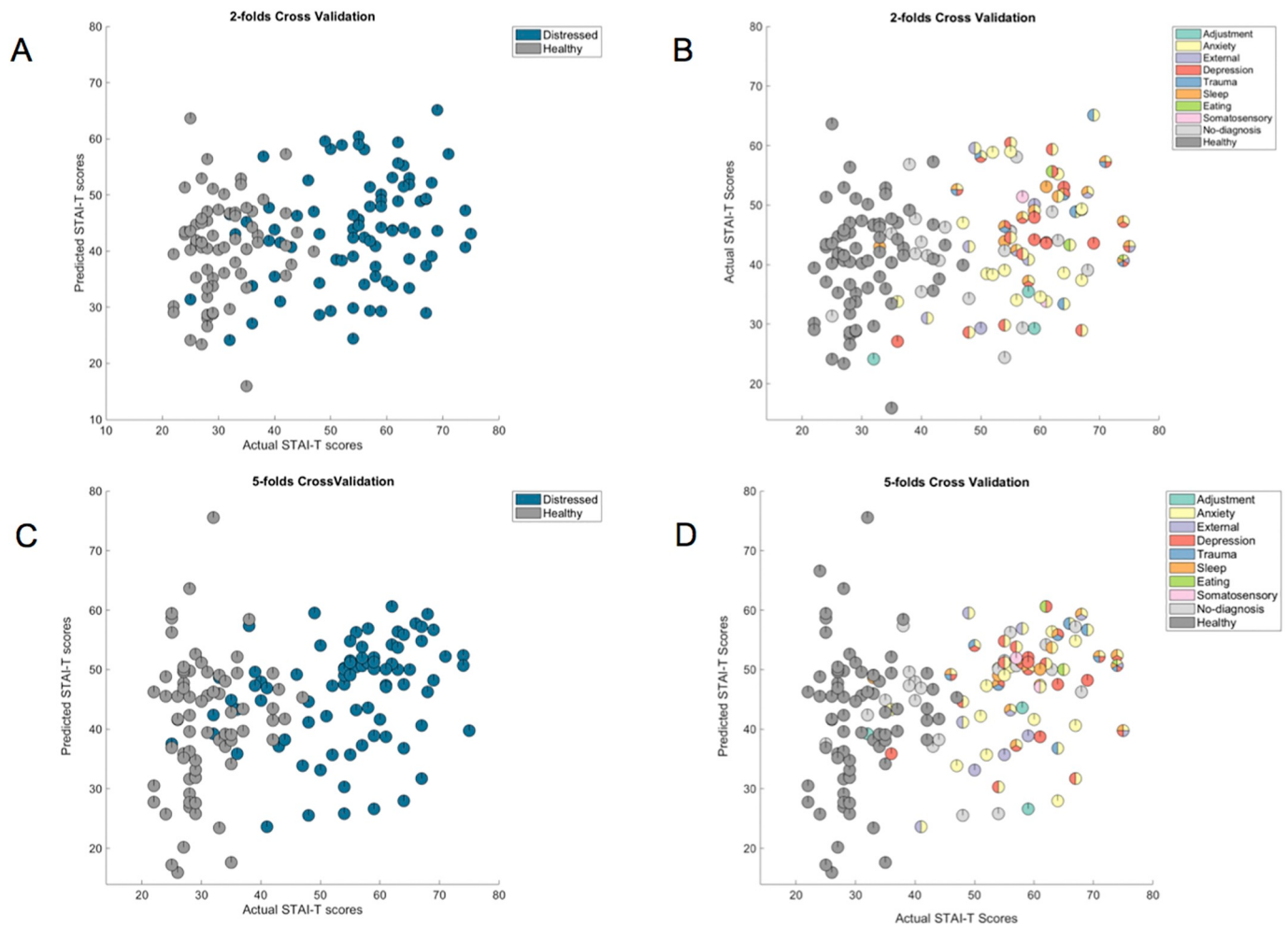
Fig. 1. (A) Scatter plot between the actual and predicted STAI-T scores for the model based on patterns of brain activation to dynamic emotional face processing in the whole sample applying a two-folds cross-validation scheme. For visualization purposes the subjects were colour coded as belonging to the healthy and distressed samples. (B) Same plot as in (A) but for visualization purposes the subjects were colour coded according to the categorically-defined diagnoses. (C) Scatter plot between the actual and predicted STAI-T scores for the model based on patterns of brain activation to dynamic emotional face processing in the whole sample applying a five-folds cross-validation scheme. Again, for visualization purposes subjects were colour coded as belonging to the healthy and distressed samples. (D) Same plot as in (C) but for visualization purposes the subjects were colour coded according to the categorically-defined diagnoses. Distressed individuals below threshold for any disorder were labelled as 'no-diagnosis'.
