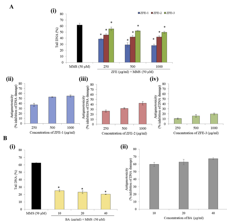
Fig. 4. A. (i) DNA damage measured as Tail DNA % in human lymphocytes exposed to MMS (50 \mu M) in combination with Ziziphus jujuba fruit extract (ZFE)-ZFE-1, ZFE-2 and ZFE-3; Antigenotoxicity of ZFE against MMS (50 \mu M) measured as % inhibition of DNA damage by (ii) ZFE-1 (iii) ZFE-2 and (iv) ZFE-3; B. (i) DNA damage measured as Tail DNA % in human lymphocytes exposed to MMS (50 \mu M) in combination with BA (10, 20, 40 \mu g/ml); (ii) Antigenotoxicity of BA against MMS (50 \mu M) measured as % inhibition of DNA damage. (* Significant with respect to MMS, p \leq 0.05 ; Error bar represents \pm SEM).
