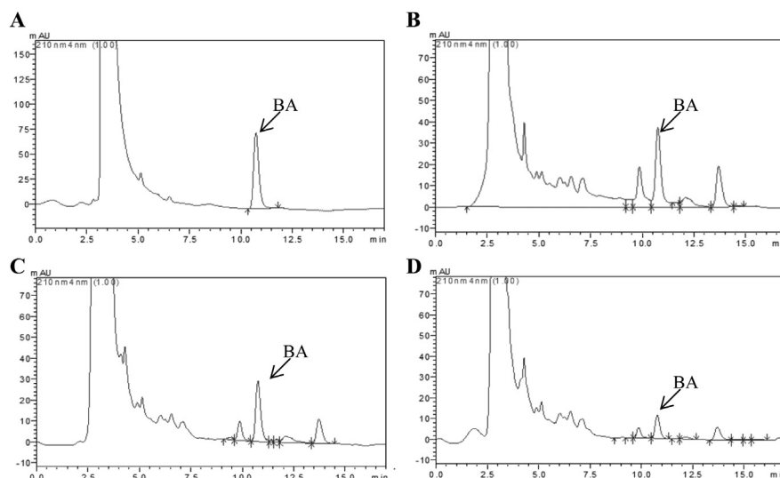
Fig. 1. HPLC-DAD chromatogram and quantification of betulinic acid (BA) in Ziziphus jujuba fruit extract (ZFE): ZFE-1 (100% ethanol), ZFE-2 (75% ethanol) and ZFE-3 (50% ethanol). (A) BA standard (B) ZFE-1 (C) ZFE-2 (D) ZFE-3. Chromatographic conditions: Agilent Eclipse plus C-18 column (150 mm × 4.6 mm, 3.5 μm), acetonitrile: water (86:14), λ = 210 nm, 0.5 ml/min flow rate.
