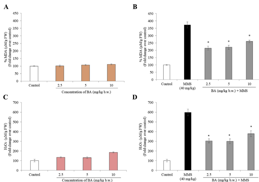
Fig. 7. Biochemical stress markers in liver cells of mice primed with betulinic acid (BA) and treated with MMS: MDA (A) BA, (B) BA followed by MMS treatment; \text{H}_2\text{O}_2 in (C) BA, (D) BA followed by MMS treatment. (* Significant with respect to MMS, p < 0.05 ; Error bar represents \pm\text{SEM} ).
