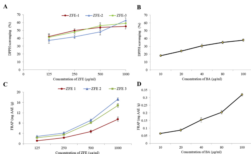
Fig. 2. Antioxidant activity of Ziziphus jujuba fruit extract (ZFE): ZFE-1 (100% ethanol), ZFE-2 (75% ethanol), ZFE-3 (50% ethanol) and betulinic acid (BA): DPPH free radical scavenging assay (A) ZFE-1, ZFE-2, ZFE-3 and (B) BA; FRAP assay (C) ZFE-1, ZFE-2, ZFE-3 and (D) BA. Results represent mean ± SEM of three independent experiments performed in triplicates.
