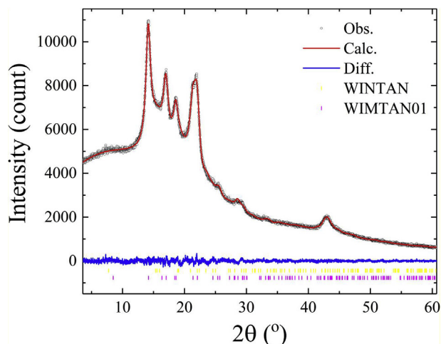
Fig. 4. Rietveld plot of PP, using the CIF files: PP \alpha_1 form (CSD: WINTAN) and \alpha_2 form (CSD: WINTAN01). The observed pattern is indicated by the black circles and the calculated one is represented by the red line. Their difference is displayed by the blue line and the positions of the Bragg peaks of the different phases are indicated by the vertical bars at the bottom of the figure. Weighted profile R-factor ( R_{wp} ) and goodness-of-fit indicator (Gof) are [25]: R_{wp} = 1.74\% and Gof = 0.99.
