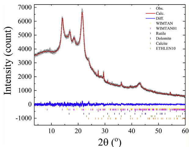
Fig. 5. Rietveld plot of PPr, using the CIF files: PP \alpha_1 form (CSD: WINTAN), \alpha_2 form (CSD: WINTAN01) and polyethylene (CSD: ETHLEN10); rutile (ICSD: 33838), dolomite (ICSD: 31209) and calcite (ICSD: 86161). The observed pattern is indicated by the black circles and the calculated one is represented by the red line. Their difference is displayed by the blue line and the positions of the Bragg peaks of the different phases are indicated by the vertical bars at the bottom of the figure. Weighted profile R-factor ( R_{wp} ) and goodness-of-fit indicator (Gof) are: R_{wp} = 1.93\% and Gof = 0.94.
