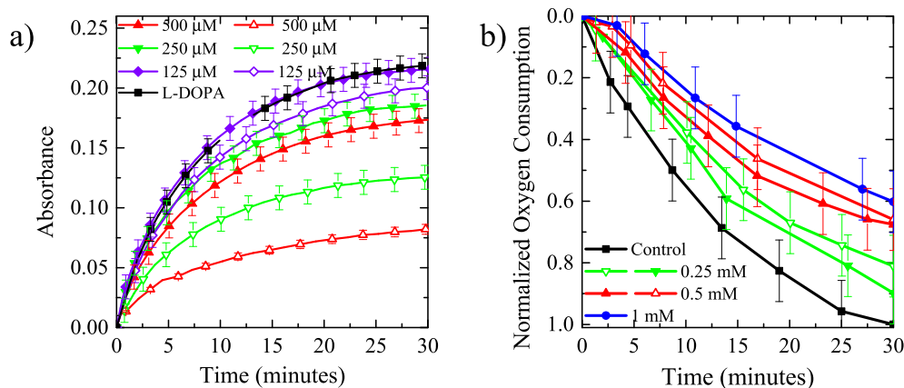
Fig. 5. UV-Vis absorption at 475 nm (a) oxygen consumption (b) of 500 \mu M of L-DOPA with tyrosinase decanal at 125 \mu M, 250 \mu M, 500 \mu M or 1 mM.
