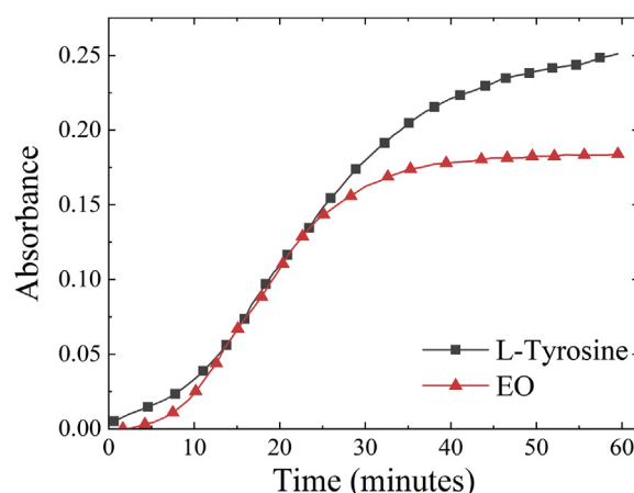
Fig. 2. Oxygen consumption of the oxidation of 500 \mu\text{M} of L-Tyrosine and essential oil at 100 \mu\text{g/mL} .
