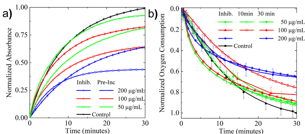
Fig. 1. UV-Vis absorption at 475 nm (a) and oxygen consumption (b) of 500 \mu\text{M} of L-DOPA with tyrosinase with essential oil (50 \mu\text{g/mL} , 100 \mu\text{g/mL} , 200 \mu\text{g/mL} ).
