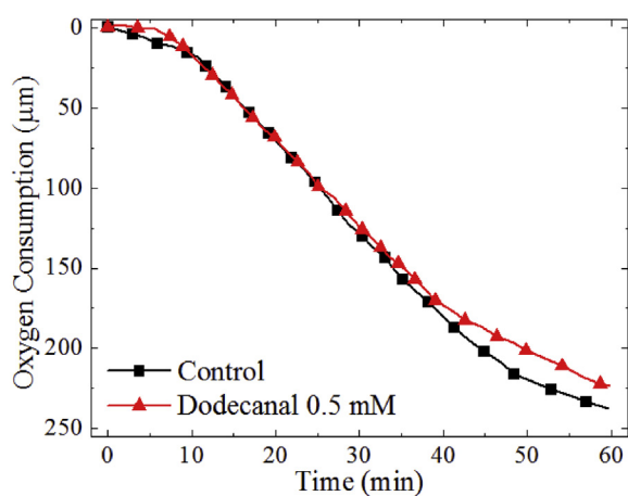
Fig. 4. Oxygen consumption of the oxidation of 500 \mu M of L-tyrosine and dodecanal at 500 \mu M.
