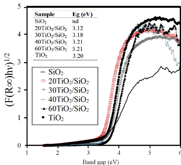
Fig. 5. DRS spectra of materials.
