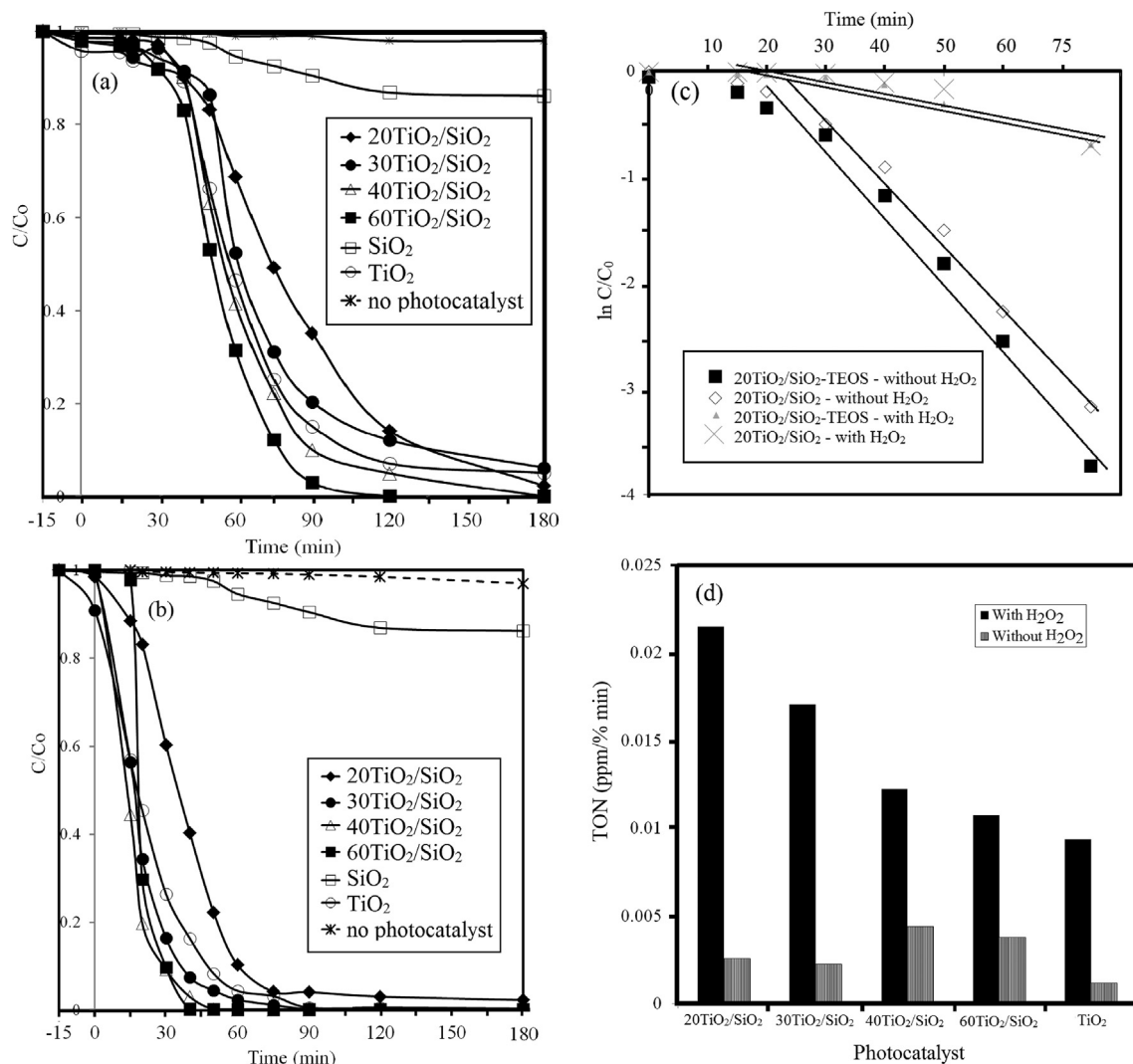
Fig. 6. (a) Kinetics of MB photocatalytic degradation without H_2O_2 addition (b) Kinetics of MB photocatalytic degradation with H_2O_2 addition (c) pseudo-first order plot of MB photocatalytic degradation using 20TiO 2 /SiO 2 and 20TiO 2 /SiO 2 -TEOS (d) TON of photocatalytic degradation over varied photocatalysts.
