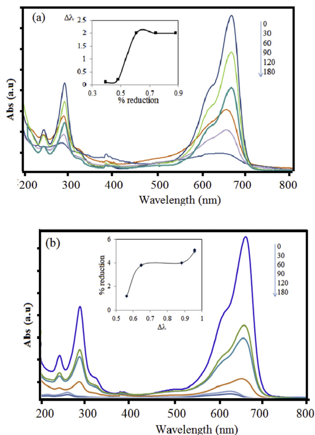
Fig. 8. UV-Vis spectra of treated MB solution by photocatalytic degradation (a) without \text{H}_2\text{O}_2 addition (b) without \text{H}_2\text{O}_2 addition.
