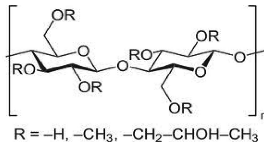
Fig. 3. Structure of HPMC.
