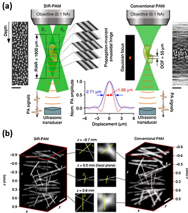
Fig. 5. Motionless SIR-PAM vs. conventional OR-PAM. (a) The concept and the measured lateral resolution, RIRAR, and DoF (b) Volume-rendered images of carbon fibers. PAM, photoacoustic microscopy; SIR-PAM, spatially invariant resolution PAM; OR-PAM, optical-resolution PAM; E_1 and E_2 , symmetrical plane waves of the propagation-invariant sinusoidal fringes; RIRAR, resolution-invariant axial range; and DoF, depth of field. Reproduced with permission from Ref. [70].
