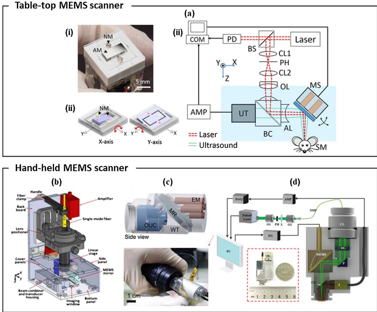
Fig. 7. (a) (i) Photograph, (ii) scanning mirror schematic, and (iii) system setup of the 2-axis MEMS scanner OR-PAM. NM, neodymium magnet; AM, aluminum mirror; COM, computer; PD, photodiode; BS, beam splitter; AMP, amplifier; UT, ultrasound transducer; CL, condenser lens; PH, pinhole; OL, objective lens; BC, beam combiner; AL, acoustic lens; MS, MEMS scanner; and SM, sample; and CPL, carbon particles lump. (b) Handheld OR-PAM system using a 1-axis MEMS scanner. (c) Scanner schematic (top) and photograph (bottom) of handheld PAM with a 2-axis MEMS scanner. EM, electromagnets; MR, mirror; OUC, opto-ultrasound combiner; and WT, water tank. (d) Schematic of an ultra-compact portable PAM with a 2-axis MEMS scanner. O, objective lens; DAQ, data acquisition card; L, convex lens; SMF, single-mode fiber; CL, collimation lens; DL, doublet lens; P, prism; CG, cover glass; FG, function generator; T, transducer; MEMS, micro-electro-mechanical system; and OR-PAM, optical-resolution photoacoustic microscopy. Reproduced with permission from Ref. [82–85].
