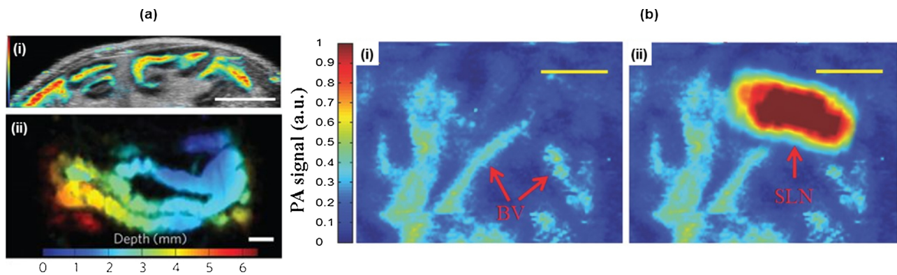
Fig. 13. (a) AR-PAM (color) and ultrasound (grey) B mode image (i) and depth-encoded AR-PAM MAP image (ii) of mouse intestine after injection of ZnBNC nanonaps. Scale bar: 5 mm (b) AR-PAM MAP images of SLN before (i) and after (ii) injection of N4 NPs. Scale bar: 1 mm. AR-PAM, acoustic-resolution photoacoustic microscopy; MAP, maximum amplitude projection; SLN, sentinel lymph node; and NP, nanoparticle. Reproduced with permission from Ref. [16,119].
