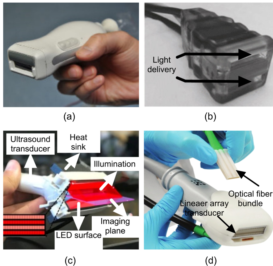
Fig. 9. Linear array transducers used in photoacoustic signal detection, (a) Reproduced with permission from Ref. [104], (b) Reproduced with permission from Ref. [18], (c) Reproduced with permission from Ref. [67], and (d) Visualsonic PA probe. Reproduced with permission from Fujifilm VisualSonics Inc.
