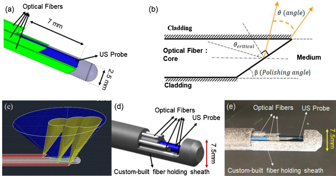
Fig. 1. (a) Schematic of designed PA/US endoscope with optical fibers (shown in green), (b) Side illuminating optical fiber approach based on total internal reflection (yellow lines represent the light escaping total internal confinement), (c) US transducer field of view (shown in blue) and fiber optics illumination area (shown in yellow), (d) Combined PA/US endoscope including US aperture (shown in blue), fiber optics (shown in white), and the three housing sheaths shown in gray, (e) A photograph of the assembled PA/US probe.
