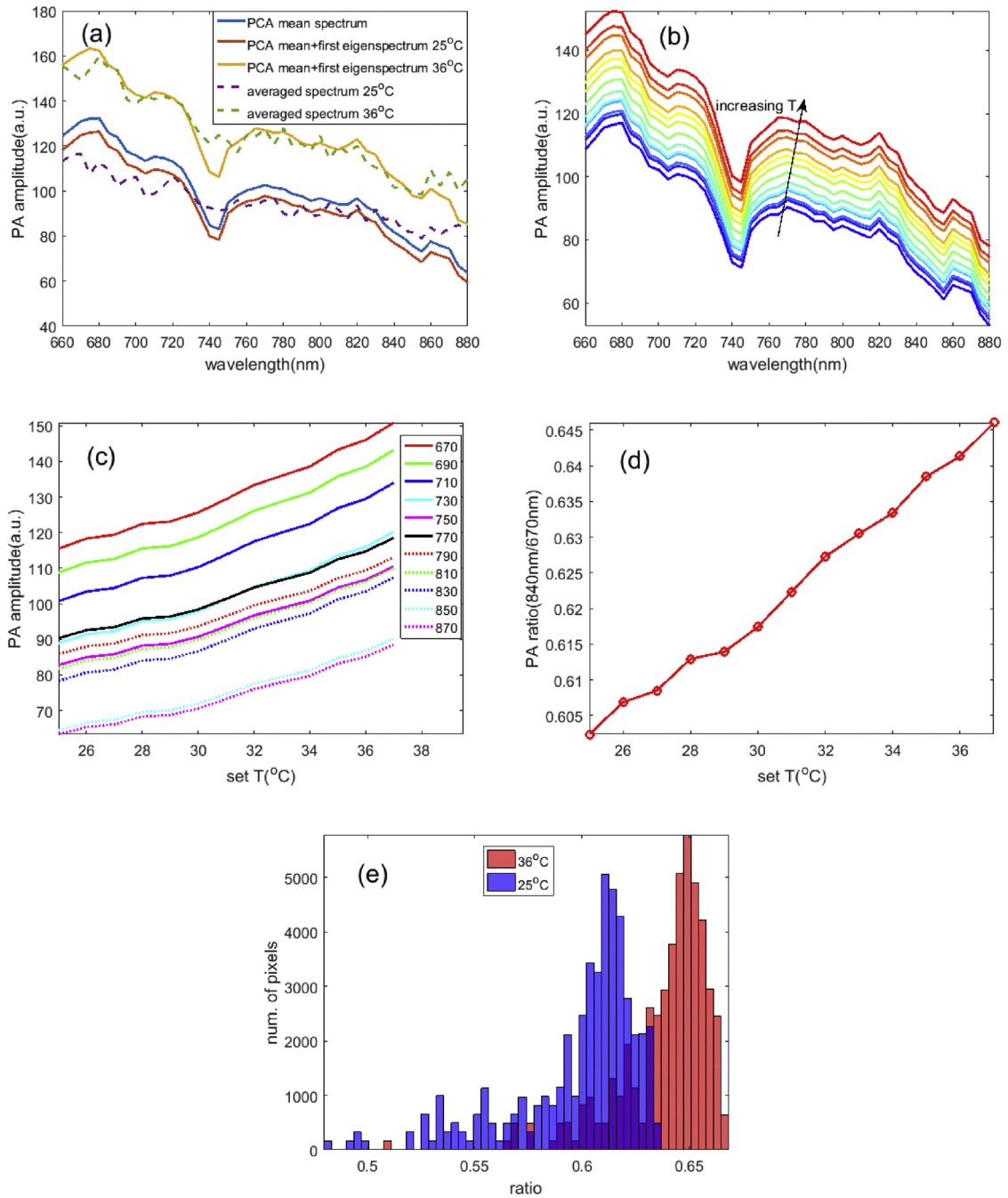
Fig. 5. (a) Comparison between the mean PCA spectrum, the PA spectra at 25 and 36 °C, spatially averaged over one region ( \theta = [0, 12^\circ] and r = [0, 3.8 \text{ mm}] ), and their largest principal component. (b) PCA-processed spectra in this region at different temperatures. (c) Corresponding amplitude variation with temperature at selected wavelengths. (d) PA ratio between 840 and 670 nm variation with temperature. (e) Statistical distribution of the PA ratio after PCA at 36 °C and 25 °C.
