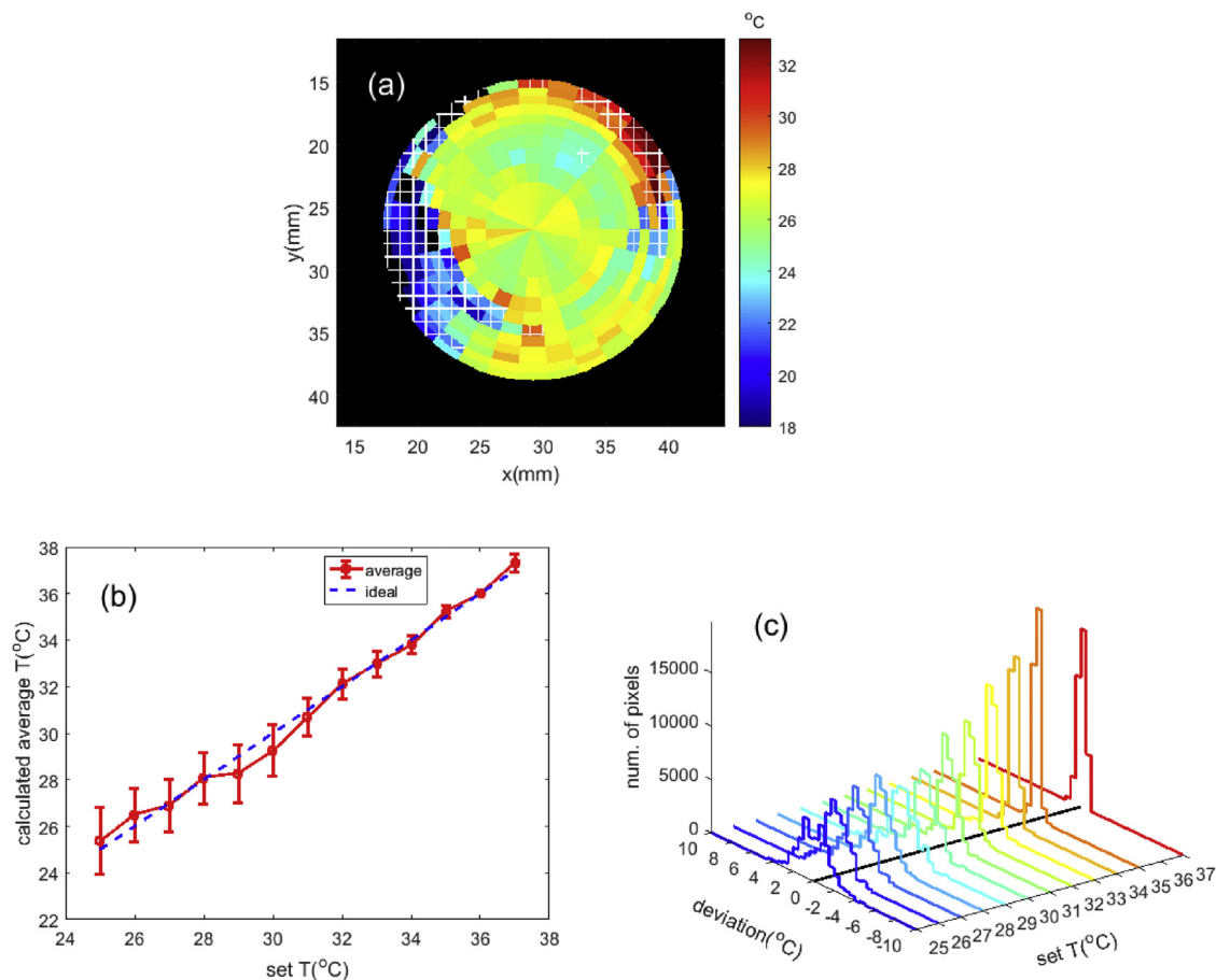
Fig. 8. Pseudo color temperature map obtained at 26 °C (a). Plots of (b) spatially averaged reconstructed temperatures versus set water bath temperature and (c) reconstructed temperature deviation distributions. The curves were obtained from the slope average over its 75% most frequent values in the ROI and with a reference temperature of 36 °C. For Figs. 7(d), 8 (c) and 9 (b), a bin size of 0.5 °C was used to calculate the distributions, and the black line at the base of the plots indicates a 0 °C deviation.
