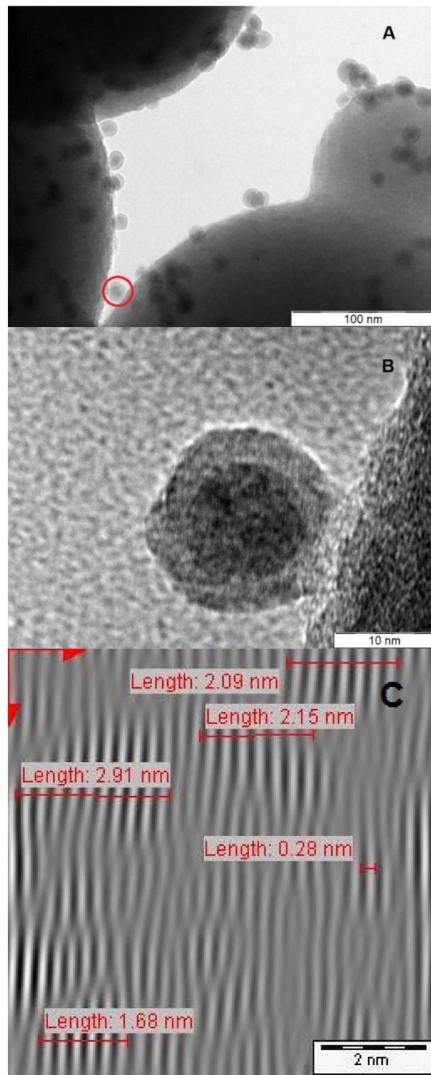
Fig. 6. TEM micrographs of Ni^0 NPs supported on MSNS by impregnation method (A), HRTEM of an isolated nanoparticle (B) and their inverse Fourier transform (C).
