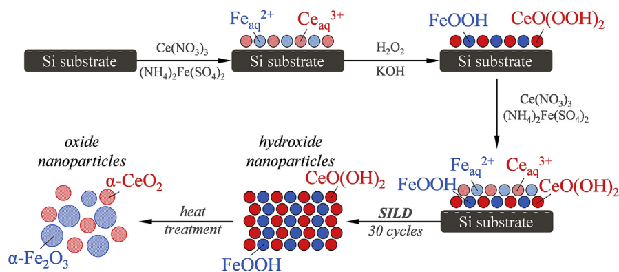
Fig. 7. Schematic representation of formation mechanism of nanocomposite of ultrafine cerium (IV) and iron (III) oxides synthesized via peroxide route of SILD.
