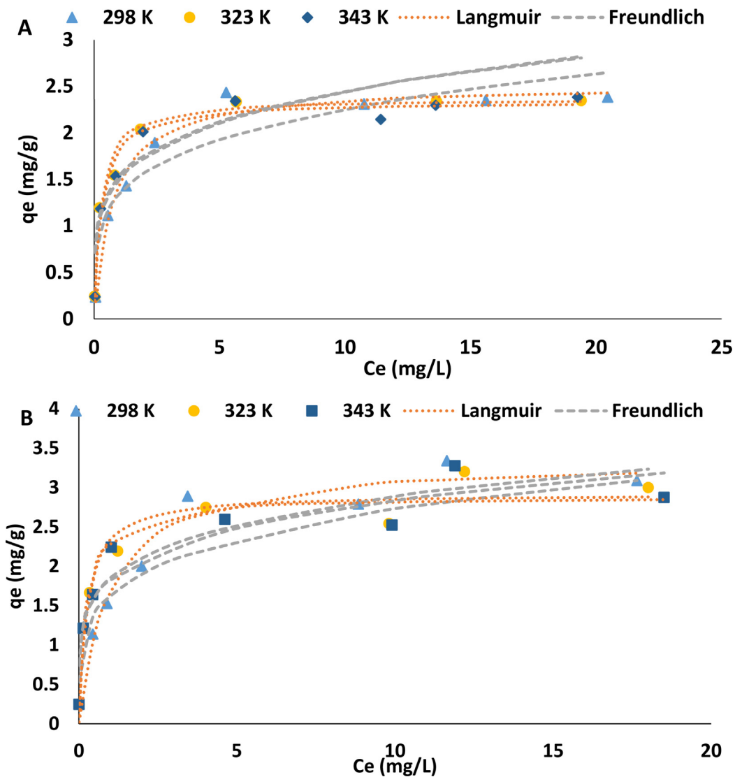
Fig. 9. Adsorption isotherms for As(III) (a) and As(V) (b) adsorption onto SMK (adsorbent dosage: 0.4 g/100 mL, pH: 6 \pm 0.5 , contact time: 60 min and shaking speed: 250 rpm).
