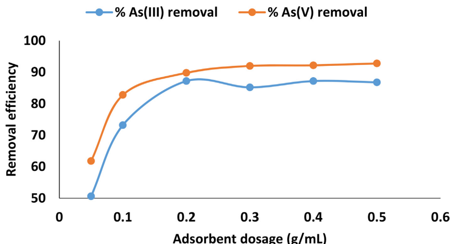
Fig. 8. Effect of adsorbent dosage on As(III) and As(V) removal (Adsorbate concentration: 5 mg/L; contact time: 60 min; shaking speed: 250 rpm; pH 6 \pm 0.5 ).
