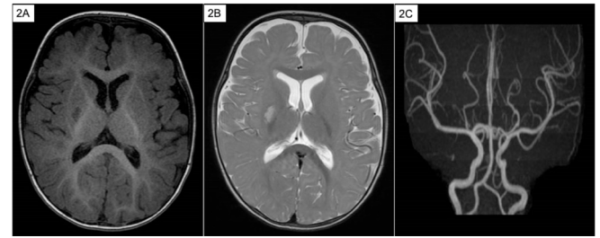
Fig. 2. Representative axial T1-weighted ( 2A ) image showing hypointense signal in the right globus pallidus and putamen region. The corresponding T2-weighted ( 2B ) MRI image shows hyperintense signal in the same region as 2A . Magnetic resonance angiography ( 2C ) demonstrates no evidence of flow-limiting stenosis. Of interest, these MRI images are incongruent with the previously described MRI findings of mineralizing microangiopathy [24]. However, these findings are also consistent with the negative MRI results seen in lenticulostriate mineralization—the subtype of mineralizing microangiopathy associated with acute basal ganglia stroke in infants presenting after minor head injury [17].
