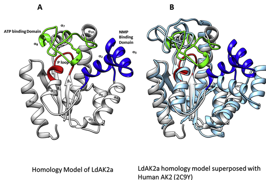
Fig. 4. Homology model and superposition of LdAK2a
