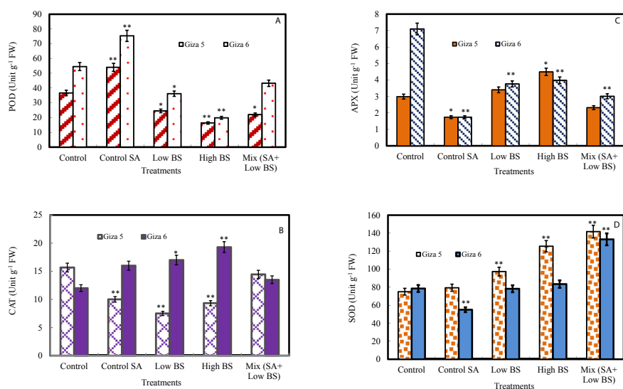
Fig. 2. Effect of Basagran ® and SA treatments on antioxidant enzyme activities of peanut ( Arachis hypogaea L. cv. G5 and G6) leaves. Peroxidase (A); Catalase (B); Ascorbate peroxidase (C); Superoxide dismutase (D).
