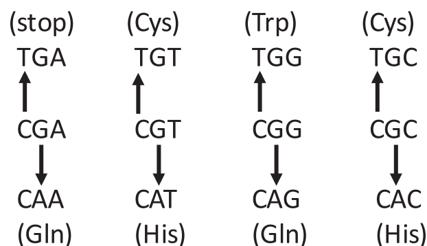
Fig. 4. Potential C•G → T•A deamination derived mutations at 5-mCpGpN codons (only coding strand shown).
