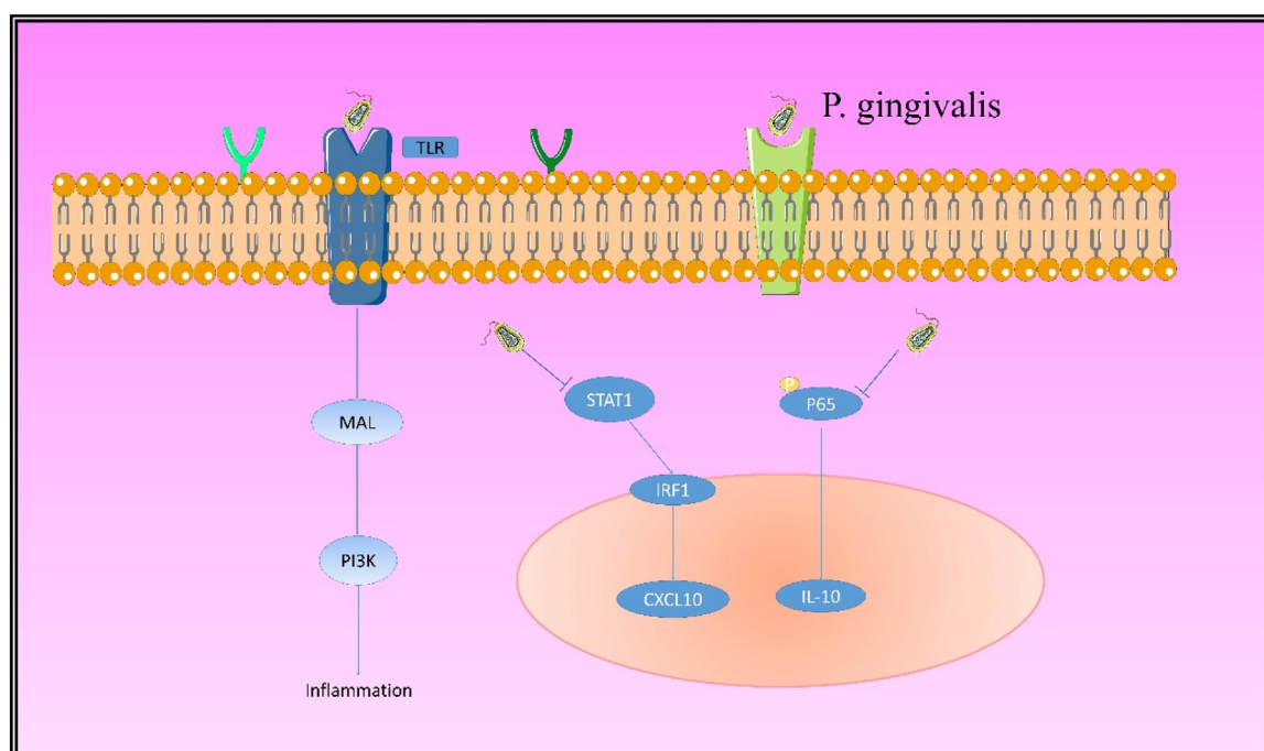
Fig. 2. Mechanism of P. gingivalis regulating inflammation in cells.
