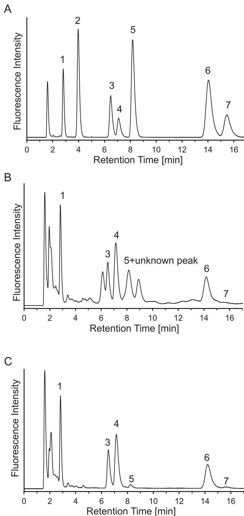
Fig. 2. Chromatogram of (A) 1 \mu M standard solution (0.1 \mu M MPG), (B) mouse serum samples with TCEP reaction at room temperature for 30 min, and (C) mouse serum samples with TCEP reaction on ice for 30 min. Peaks: 1, SBD-MPG; 2, SBD-NAC; 3, SBD-Hcy; 4, SBD-Cys; 5, SBD-CysGly; 6, SBD-GSH; 7, SBD- \gamma GluCys. Column: Inertsil Amide (150 \times 3.0 mm, 5 \mu m). Column temperature: 35 ^{\circ} C. Mobile phase: acetonitrile-40 mM ammonium formate buffer (pH 3.0) (75/25, v/v). Flow rate: 0.4 mL/min.
