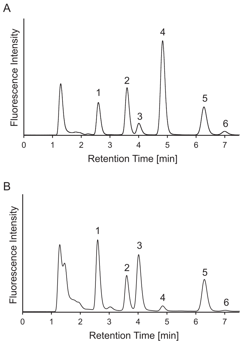
Fig. 5. Chromatograms of (A) 0.5 \mu M standard solution, and (B) mouse serum samples under the optimized conditions. Peaks: 1, SBD-NAC; 2, SBD-Hcy; 3, SBD-Cys; 4, SBD-CysGly; 5, SBD-GSH; 6, SBD- \gamma GluCys. Column: ZIC-HILIC (150 \times 2.1 mm, 3.5 \mu m). Column temperature: 35 ^{\circ} C. Mobile phase: acetonitrile-30 mM ammonium formate buffer (pH 3.4) (72/28, v/v). Flow rate: 0.3 mL/min.
