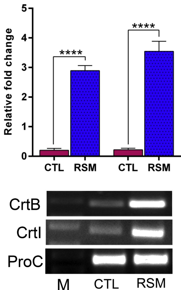
Fig. 4. Gene expression level of carotenoid biosynthetic genes for the early stationary phase cultures of E. acetylicum S01 cultivated in un-optimized medium (control) and RSM optimized medium conditions for 96 h. Data represent the mean of the three independent biological repeats ( n = 3 ). Bar graphs showing CrtI and CrtB gene expression in un-optimized medium (control) and RSM optimized medium conditions. **** p < 0.0001 indicates a significant difference between the un-optimized medium in response to RSM optimized medium conditions. Non-adjusted images provided in the supplementary material. M - DNA ladder (0.25 kb–10 kb), CTL - Un-optimized medium, RSM - RSM Optimized medium.
