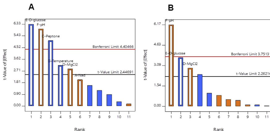
Fig. 2. Pareto chart analysis: the effect of media component on biomass (A) and \beta -carotene (B) productivities were represented by t-value.
