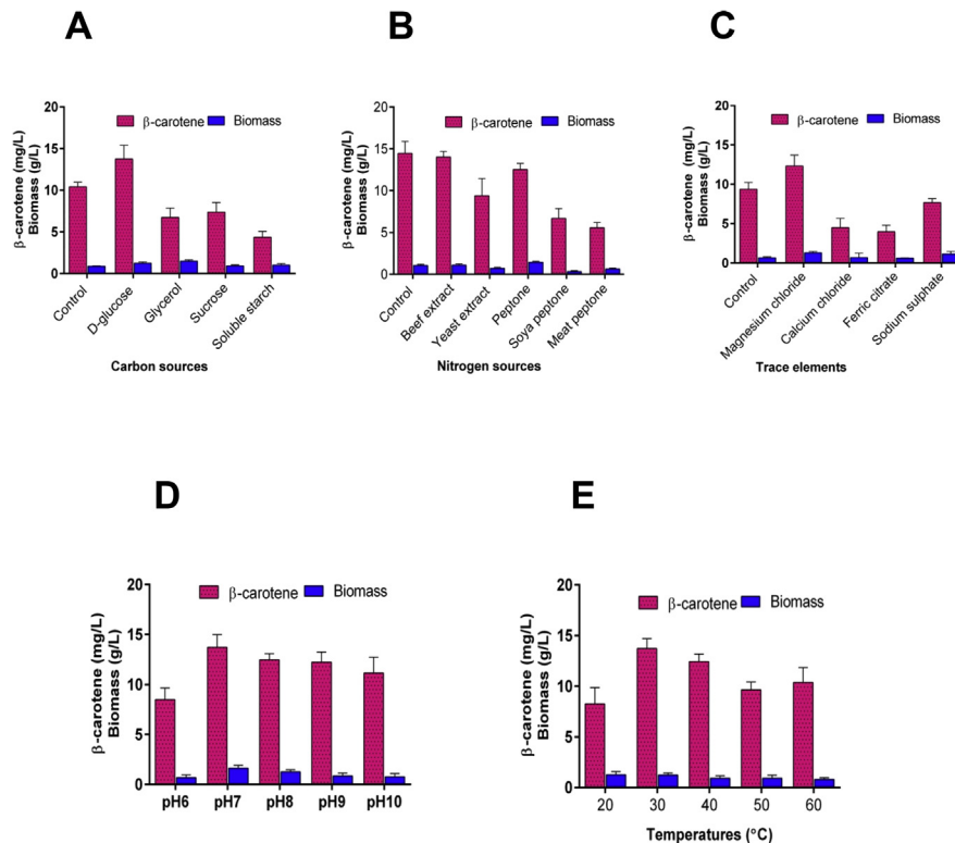
Fig. 1. Effects of different medium components and physical factors on biomass (g/L) and \beta -carotene (mg/L) productivities in E. acetylicum S01. Data are shown as mean \pm SD (n = 3). Bar graphs showing the effects of carbon source (A), nitrogen source (B), trace element (C), pH (D), and temperature (E).
