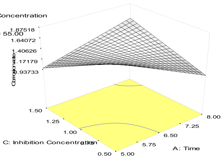
Fig. 2. Effects of time and inhibitor concentration on corrosion rate of CNE on Mild Steel at constant temperature.
