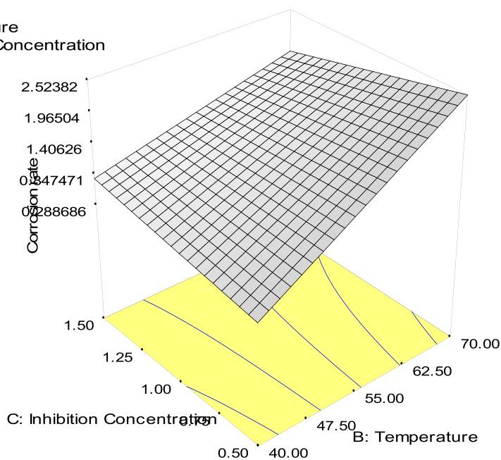
Fig. 3. Effects of temperature and inhibitor concentration on corrosion rate of CNE on Mild Steel at constant time.
