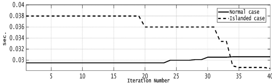
Fig. 17. Maximum latency time converge curve USING BTLBOA.
