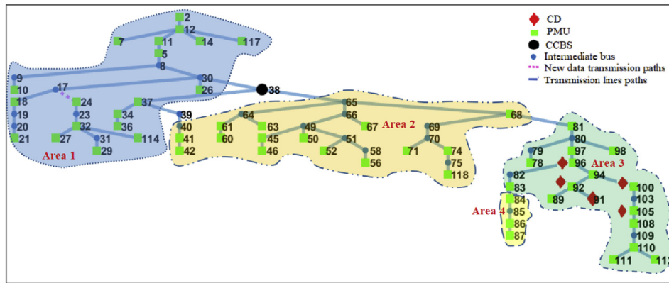
Fig. 11. Islanded case network topology USING BTLBOA Combined with MST.
