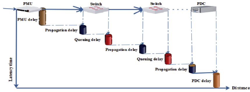
Fig. 3. Latency time.
