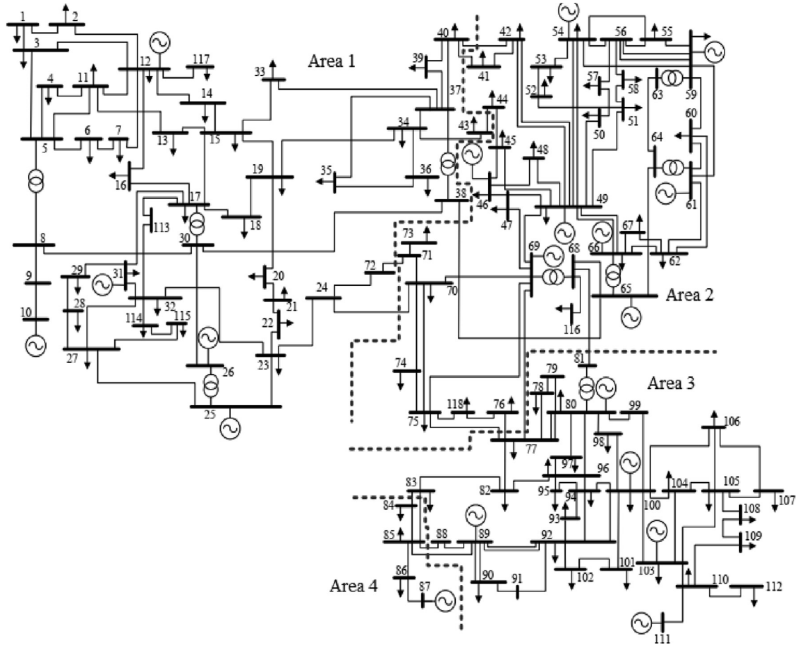
Fig. 1. IEEE 118-bus test system representing the weak connections.
