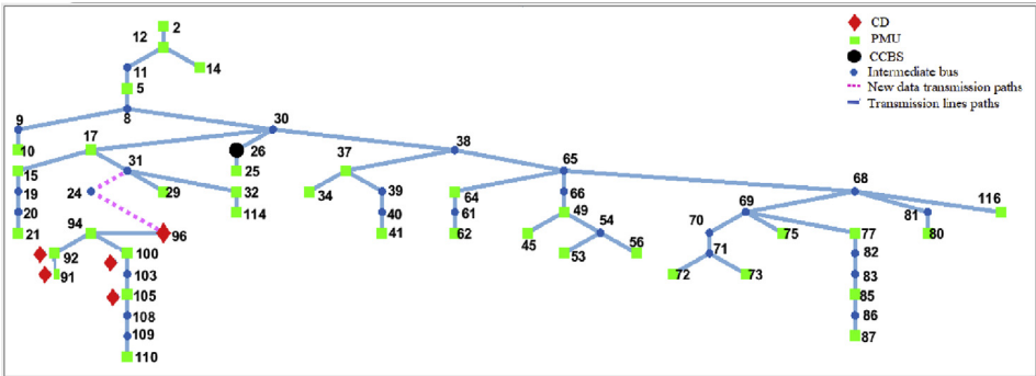
Fig. 14. Normal case network topology USING BTLBOA.
