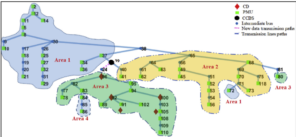
Fig. 15. Islanded case network topology USING BTLBOA.
