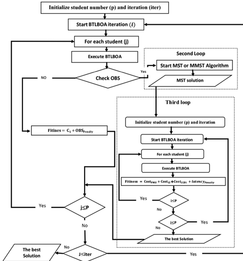
Fig. 7. Flow chart of BTLBOA and MST.
