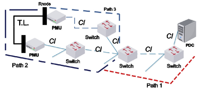
Fig. 5. Redundancy with PMU at Rnode and Nnode.
