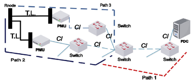
Fig. 6. Redundancy with PMUs only at Nnodes.
