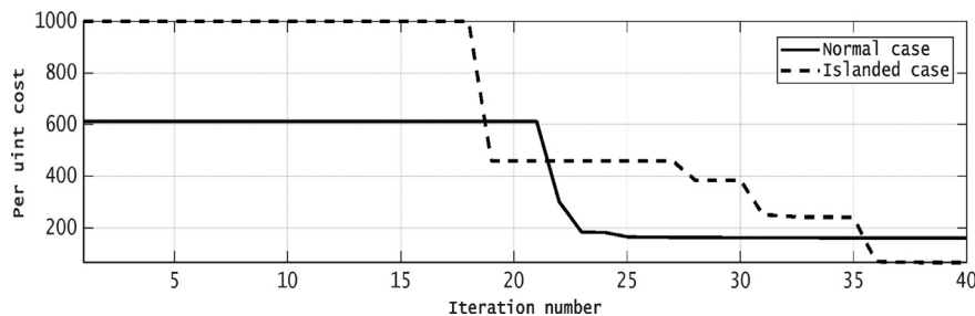
Fig. 12. Total cost converge curve USING BTLBOA Combined with MST.
