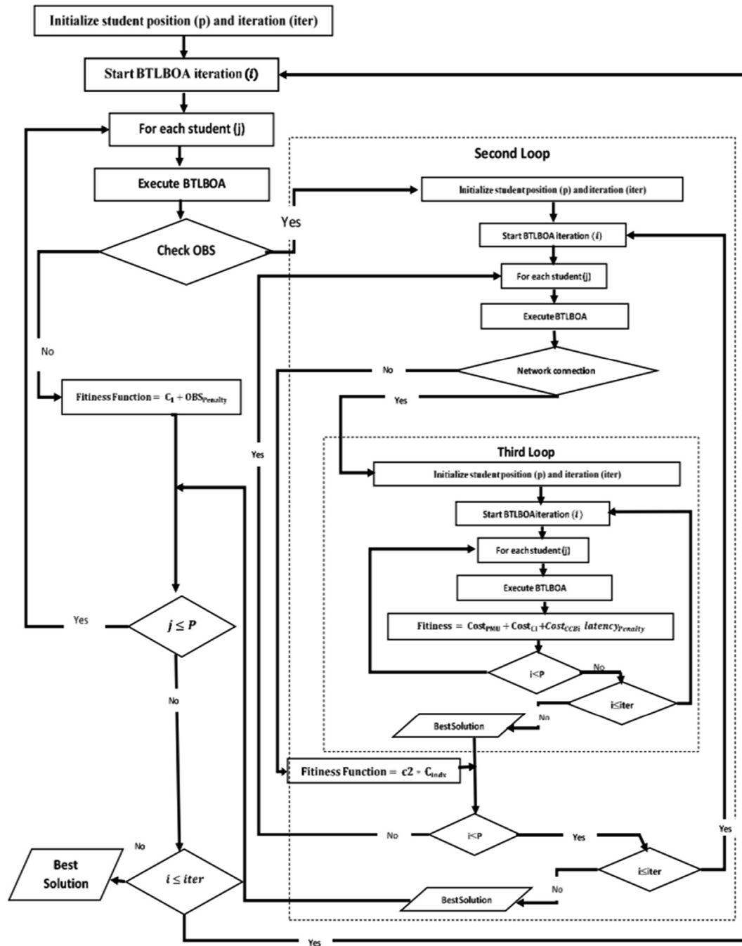
Fig. 9. Flow chart of BTLBOA.
