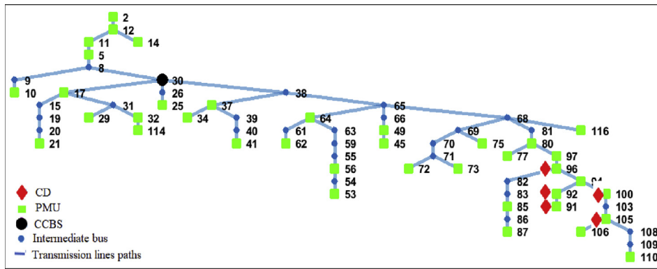
Fig. 10. Normal case network topology USING BTLBOA Combined with MST.
