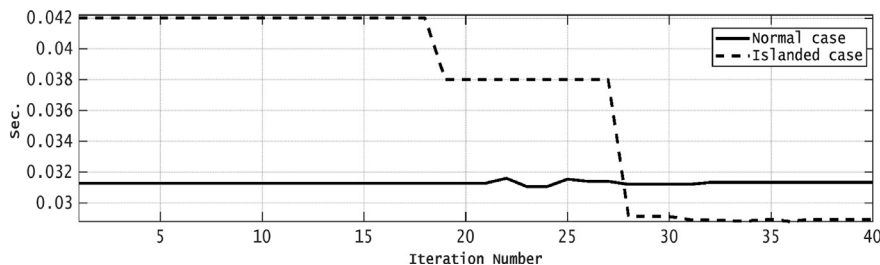
Fig. 13. Maximum latency time converge curve USING BTLBOA Combined with MST.
