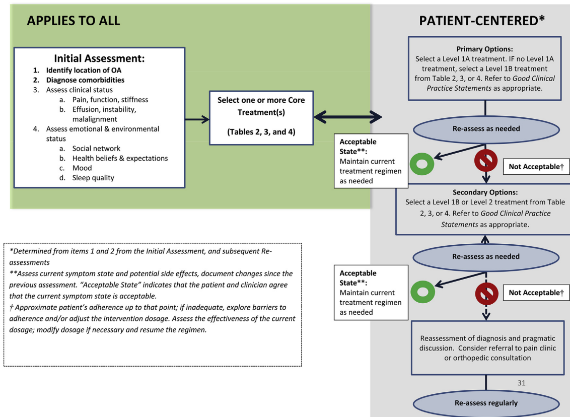
Fig. 2. Treatment algorithm.
