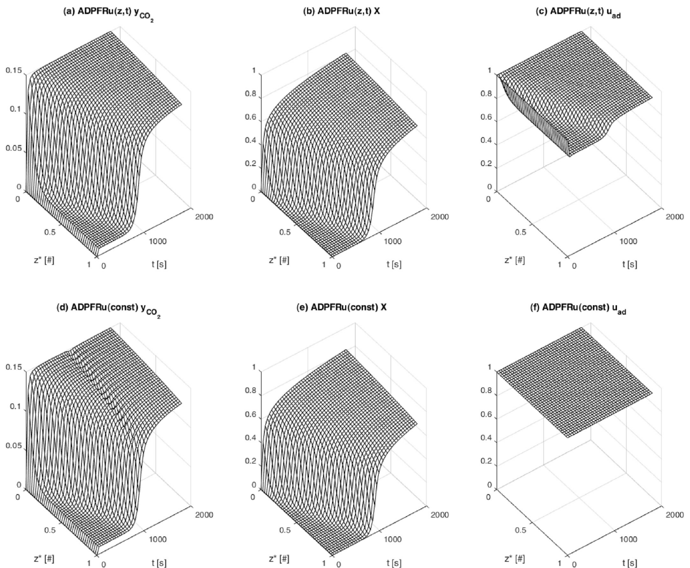
Fig. 4. Results from simulations of the case of study (with inlet CO 2 molar fraction y_{CO_2,in} = 0.15 and process duration of 1800 s) by both integration options: (a) ADPFRu(z,t) CO 2 molar fraction; (b) ADPFRu(z,t) CaO conversion; (c) ADPFRu(z,t) dimensionless superficial gas velocity; (d) ADPFRu(const) CO 2 molar fraction; (e) ADPFRu(const) CaO conversion; (f) ADPFRu(const) dimensionless superficial gas velocity.
