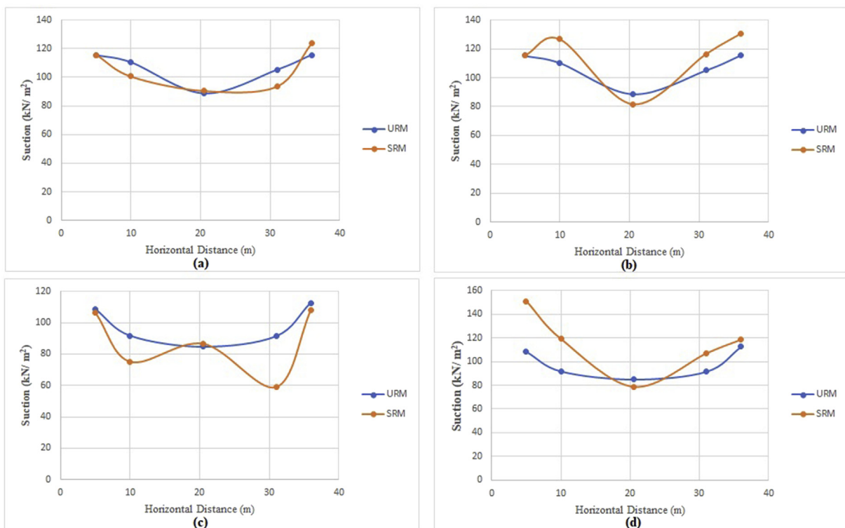
Fig. 7. Effect of buffer layer on suctions. (a) at 0.25 m depth without buffer (b) at 0.25 m depth with buffer (c) at 0.75 m depth without buffer (d) at 0.75 m depth with buffer.
