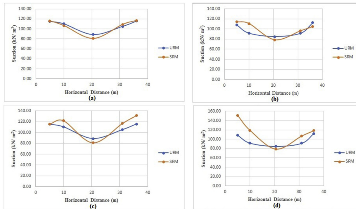
Fig. 5. Effect of volumetric strain on suctions. (a) at depth 0.25 m without volumetric strain (b) at depth 0.75 m without volumetric strain (c) at depth 0.25 m with volumetric strain (d) at depth 0.75 m with volumetric strain.
