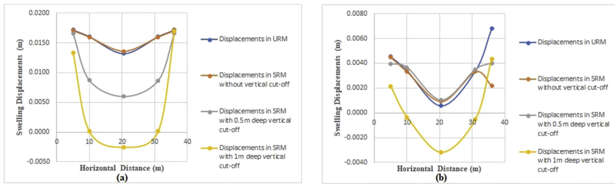
Fig. 8. Effect of vertical cut-off on vertical displacements with buffer layer present in all SRMs. (a) at 0.25 m depth (b) at 0.75 m depth.
