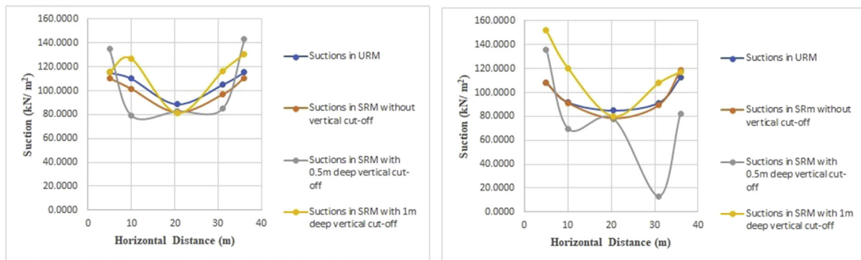
Fig. 9. Effect of vertical cut-off on suctions with buffer layer present in all SRMs. (a) at 0.25 m depth (b) at 0.75 m depth.
