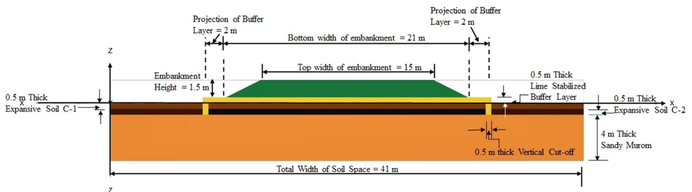
Fig. 1. Geometry of the model.
