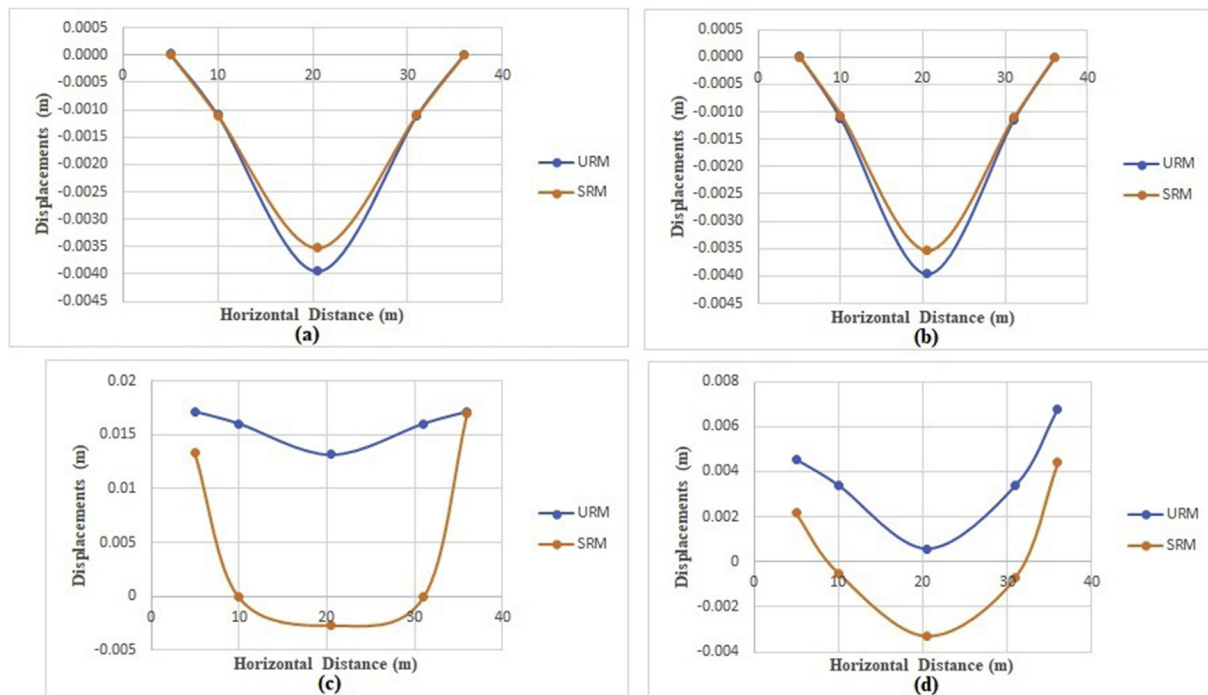
Fig. 4. Effect of volumetric strain on displacements. (a) at depth 0.25 m without volumetric strain (b) at depth 0.75 m without volumetric strain (c) at depth 0.25 m with volumetric strain (d) at depth 0.75 m with volumetric strain.
