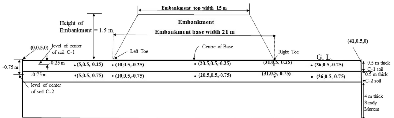
Fig. 3. Coordinates of nodes for value of swelling displacements and suctions.
