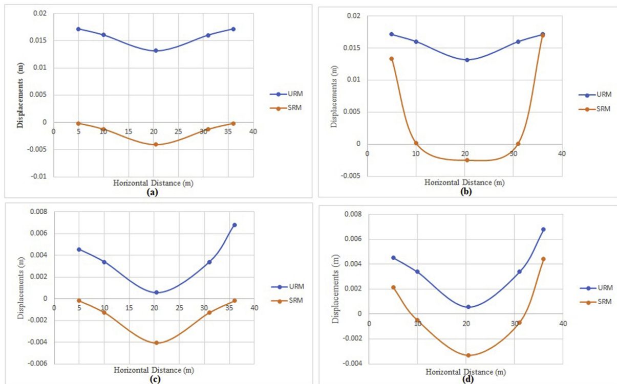
Fig. 6. Effect of buffer layer on displacements. (a) at 0.25 m depth without buffer (b) at 0.25 m depth with buffer (c) at 0.75 m depth without buffer (d) at 0.75 m depth with buffer.
