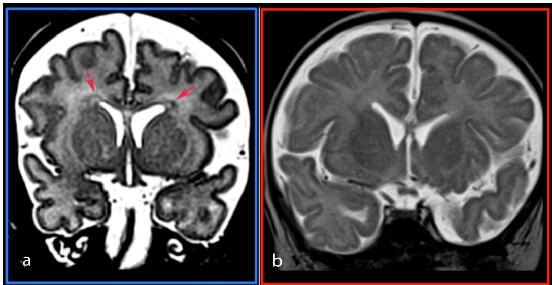
Fig. 6. Bands of migrating glial and neuronal cells. Bands of low T2w signal intensity in the deep periventricular regions of the frontal lobe (arrows in a ) indicate ongoing migration of neuronal cells. We assigned value 1 (immature) if bands of low signal intensity can be seen in the frontal periventricular white matter. If the bands of migrating cells were not visible ( b ) we assigned a value 2 (mature).
