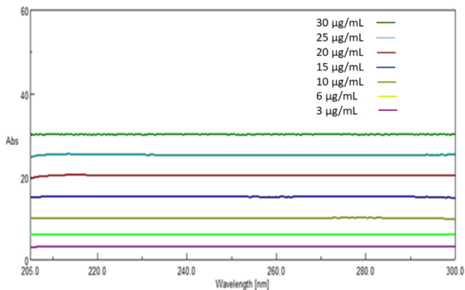
Fig. 6. The constant value gained by dividing the zero order spectra of [PHN] (3.0–30.0 \mu\text{g/mL} ) by the normalized spectra (1.0 \mu\text{g/mL} of PHN).
