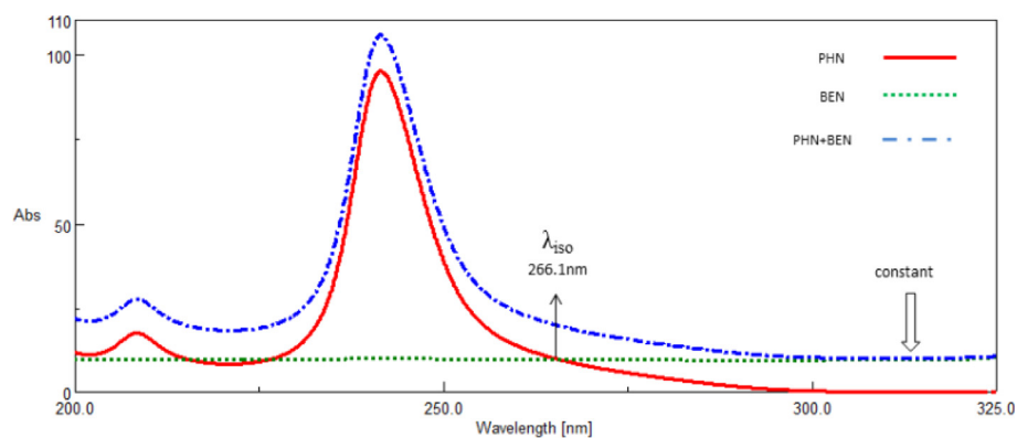
Fig. 4. Ratio spectra of 10.0 \mu\text{g/mL} of PHN, BEN separately in ethanol and their binary mixture, 10.0 \mu\text{g/mL} of each in ethanol. using the ( NS'_{\text{BEN}} ) as a divisor showing the constant region.
