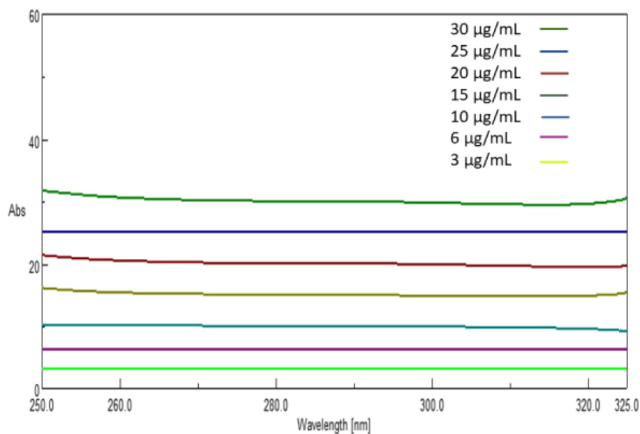
Fig. 5. The constant value gained by dividing the zero order spectra of [BEN] (3.0–30.0 \mu\text{g/mL} ) by the normalized spectra (1.0 \mu\text{g/mL} of BEN).
