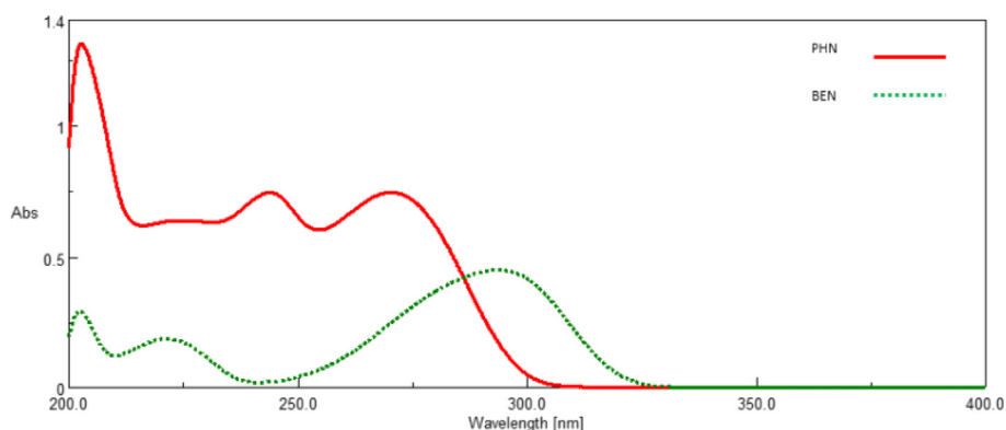
Fig. 2. Zero-order spectra of [PHN] 13.5 \mu\text{g/mL} and [BEN] 3.5 \mu\text{g/mL} in ethanol.
