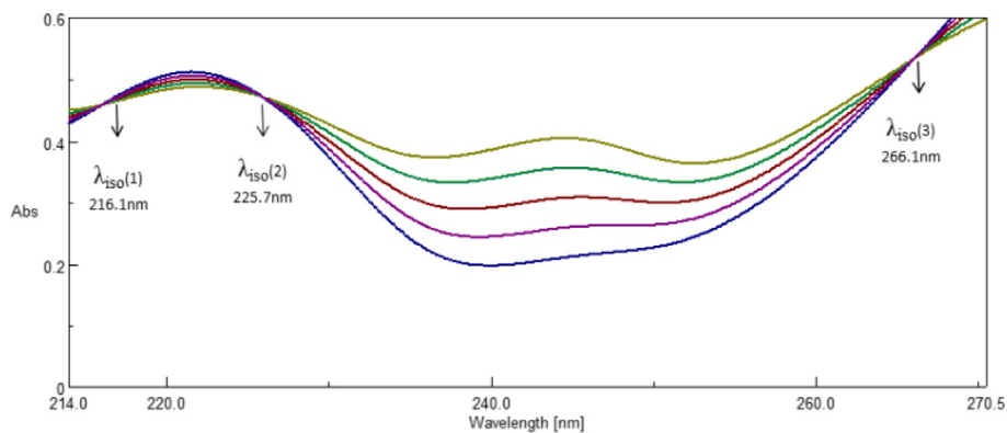
Fig. 3. Zero-order spectra of mixtures of PHN + BEN, with a total concentration equal to 10.0 \mu\text{g/mL} showing the three iso-absorptive points.
