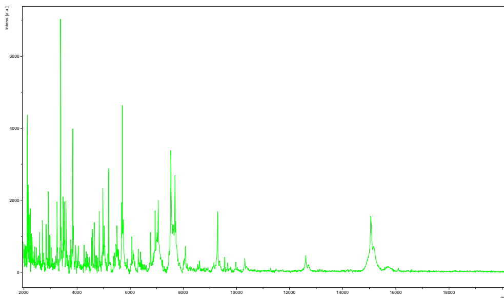
FIG. 1. MALDI-TOF MS reference mass spectrum. Spectra from 12 individual colonies were compared and a reference spectrum was generated.
