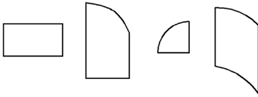
Fig. 1. Examples of decomposed domains according to Fubini's theorem. From left: a domain with 4 constant lines, a domain with 3 constant lines and 1 curve, a domain with 2 constant lines and 1 curve, and a domain with 2 parallel constant lines and 2 curves.
