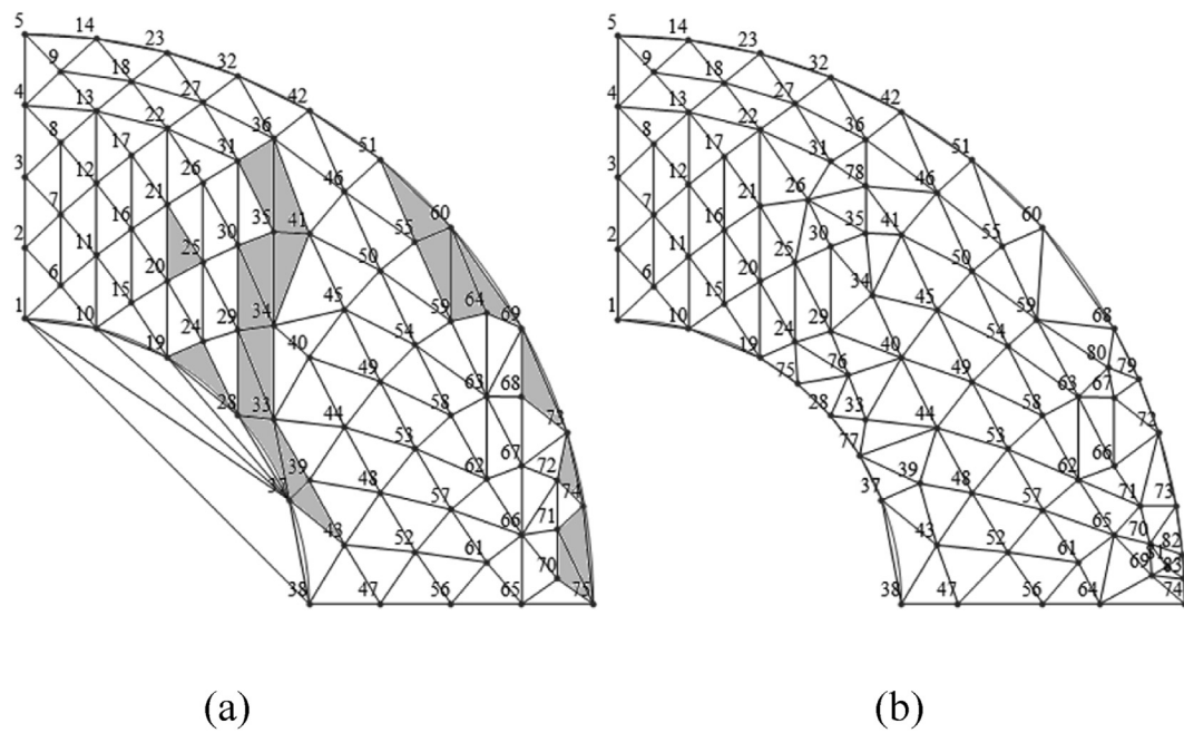
Fig. 18. Fine mesh optimisation for quadrant of hollow cylinder. (a) initial triangulation for the fine mesh associated with SP41 (b) final optimised mesh.
